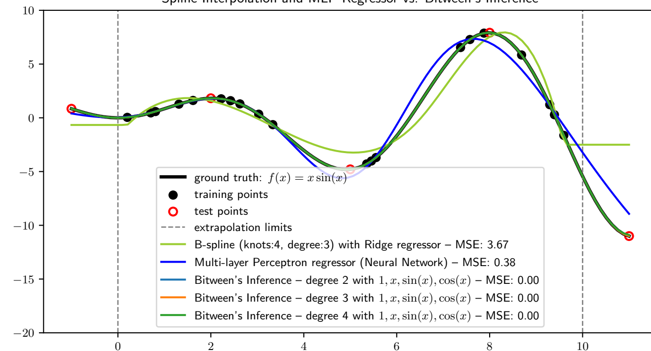
Spline Interpolation and MLP Regressor vs. Bitween's Inference
