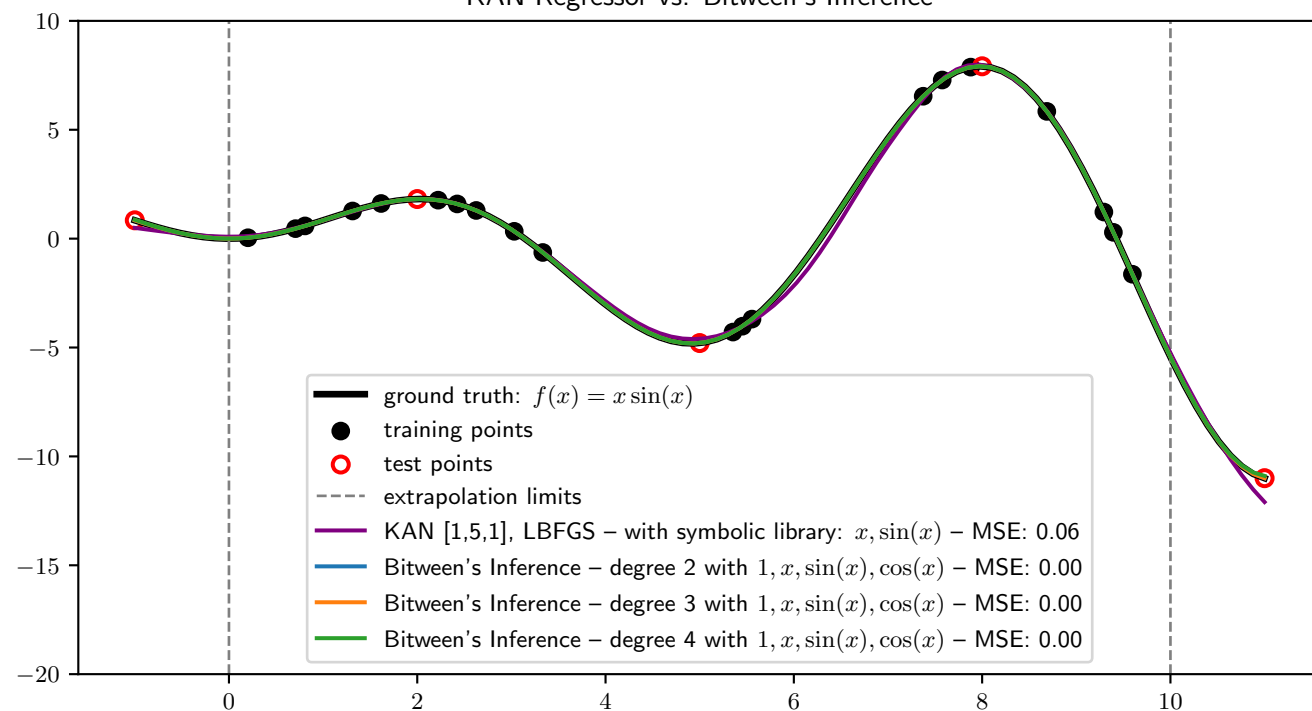
KAN Regressor vs. Bitween's Inference
