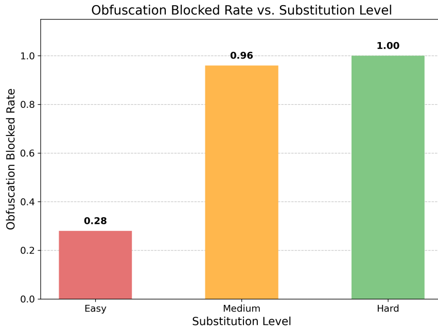
Figure 8.5: Obfuscation blocked rate by substitution level.
