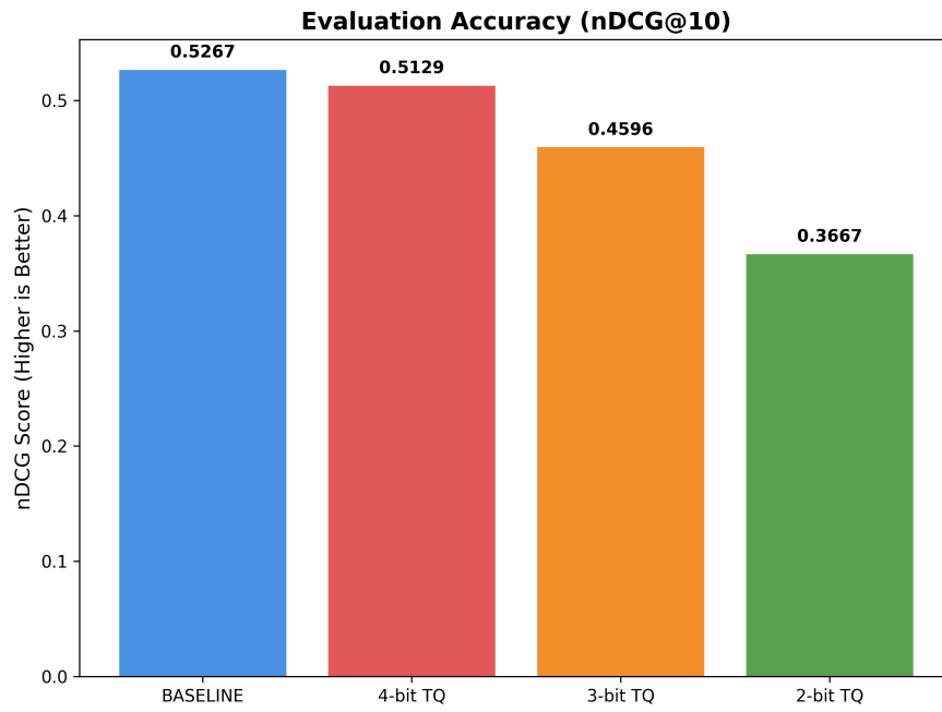
Figure 8.7: Retrieval accuracy (nDCG@10) at different quantization bit-widths.
