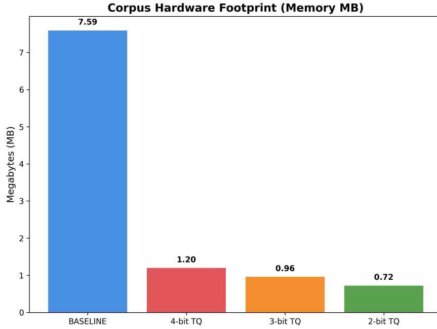
Figure 8.6: Corpus memory footprint at different quantization bit-widths.
