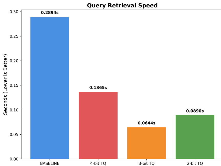
Figure 8.8: Query retrieval speed at different quantization bit-widths.
