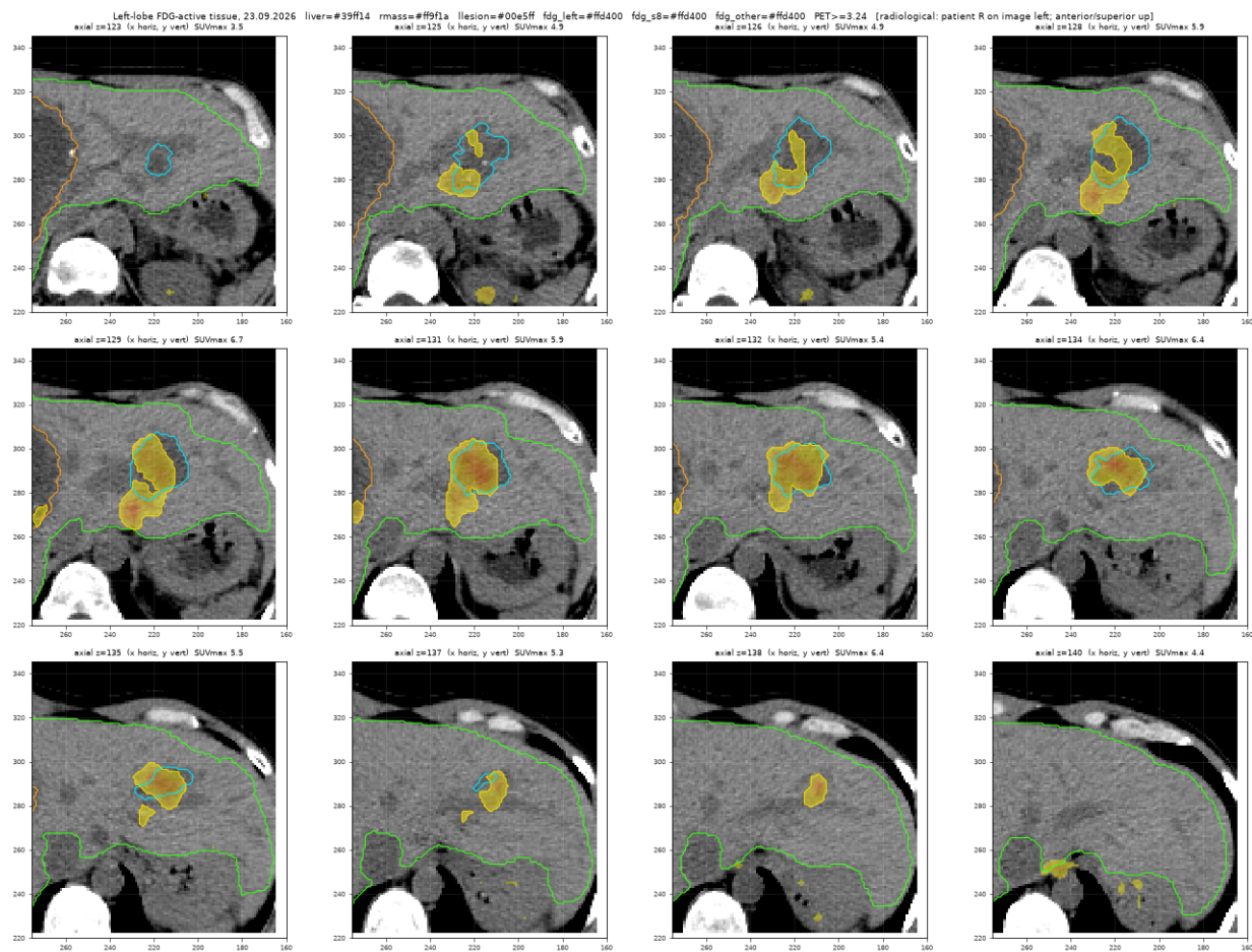
Figure 3: Left-lobe FDG-active tissue on twelve axial levels: FDG-active tissue yellow, CT lesion outline cyan, liver green; patient right on the image left, anterior up.
