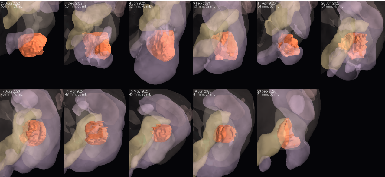
Figure 23: The same masses with ghost organs from the automatic segmentation of each study, clipped to a box around the mass: stomach (lilac), pancreas (sand), spleen (rose), liver edge (pale), left kidney (grey); bar = 5 cm.
