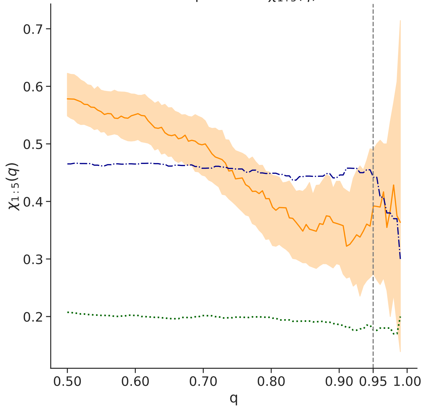
Tail Dependence \chi_{1:5}(q)
