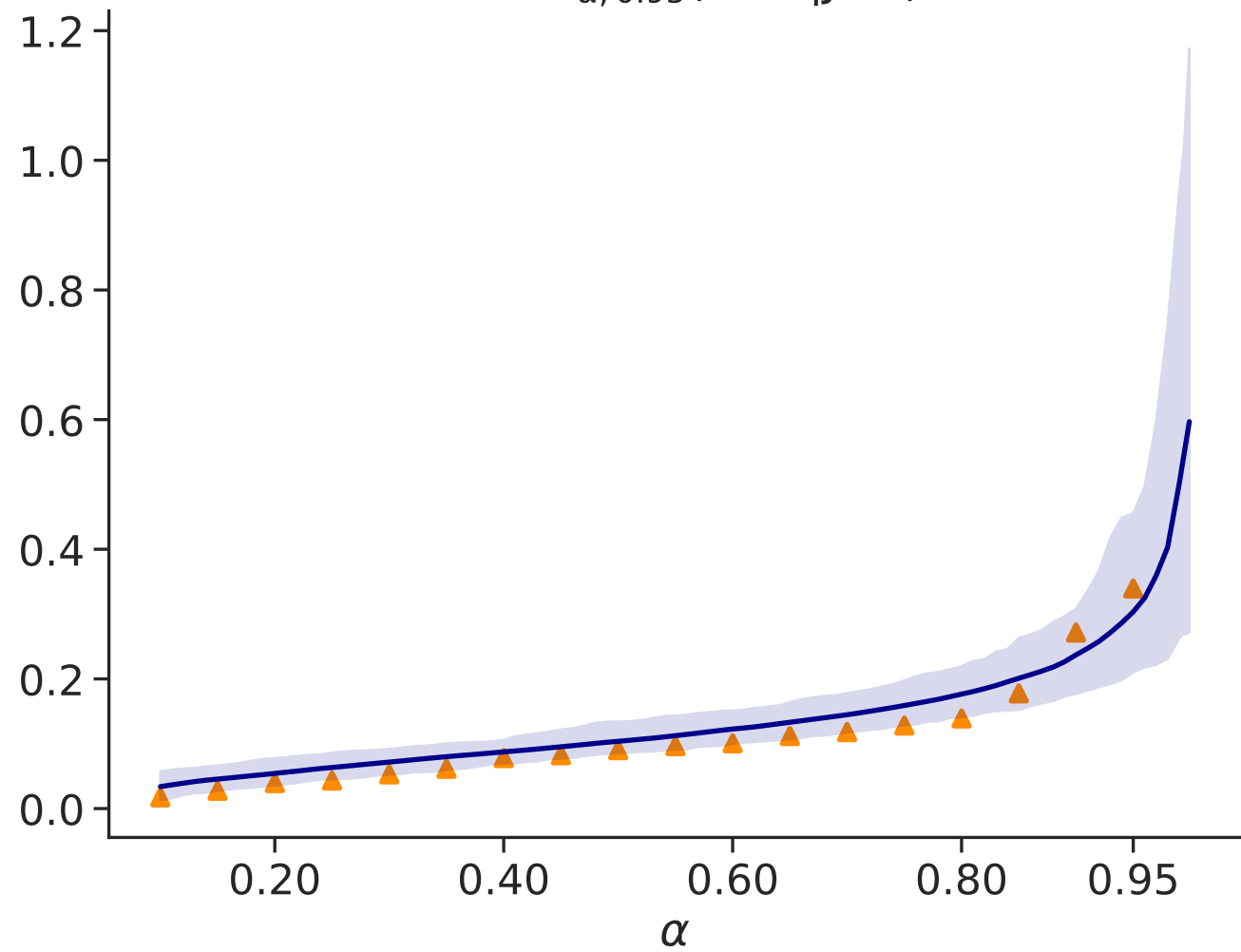
CoVaR _{\alpha, 0.95} (WFC|JPM)
