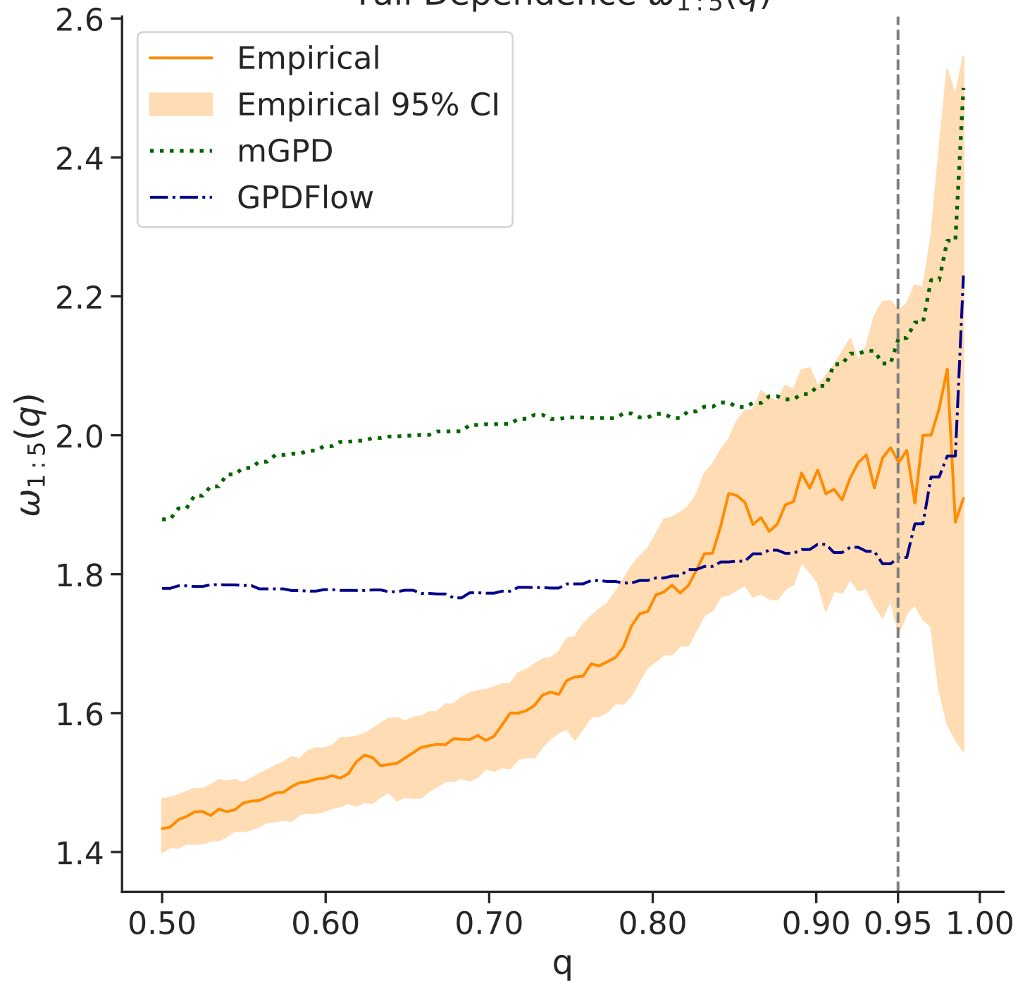
Tail Dependence \omega_{1:5}(q)
