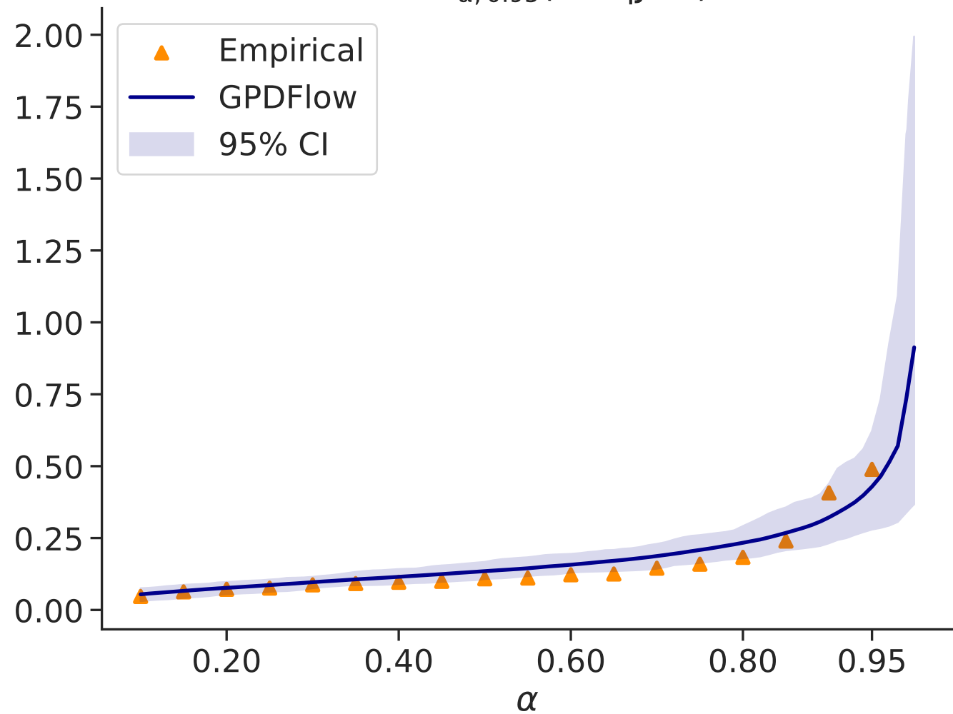
CoVaR _{\alpha, 0.95} (BAC|JPM)
