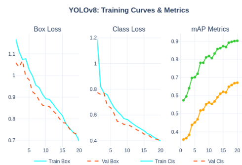
(b) Training Curves & Metrics - YOLOv8.
