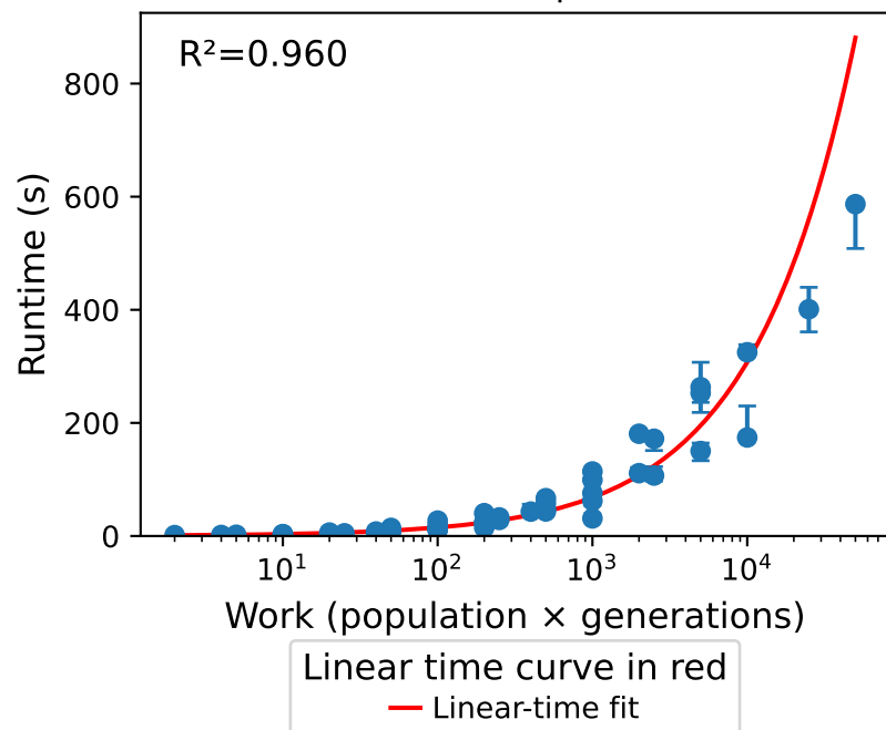
A) Runtime vs Work ( \mu=0.2 , meta=rf)
