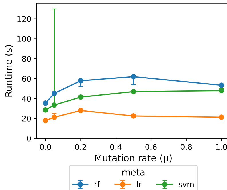
B) Runtime vs Mutation ( P=50 , G=10 )
