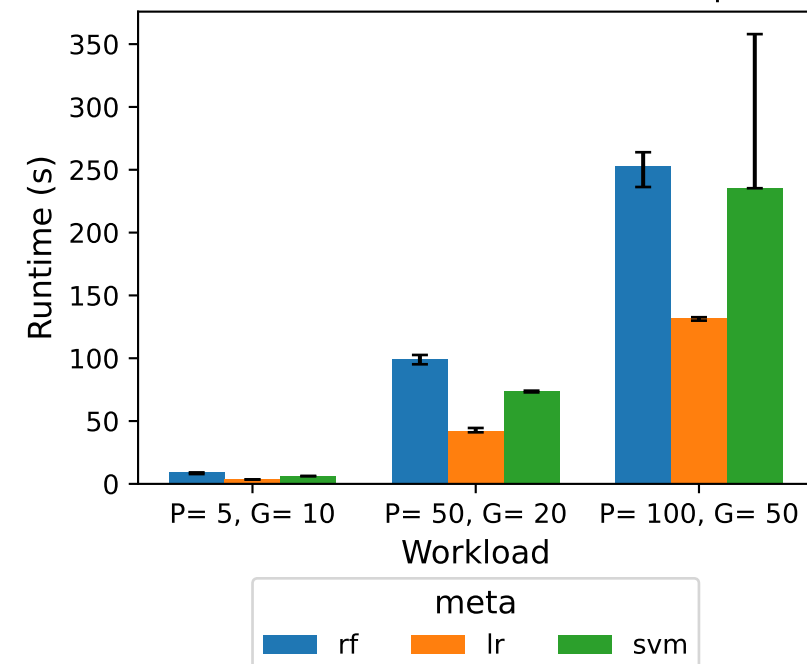
C) Runtime vs Meta at 3 Workloads ( \mu=0.2 )
