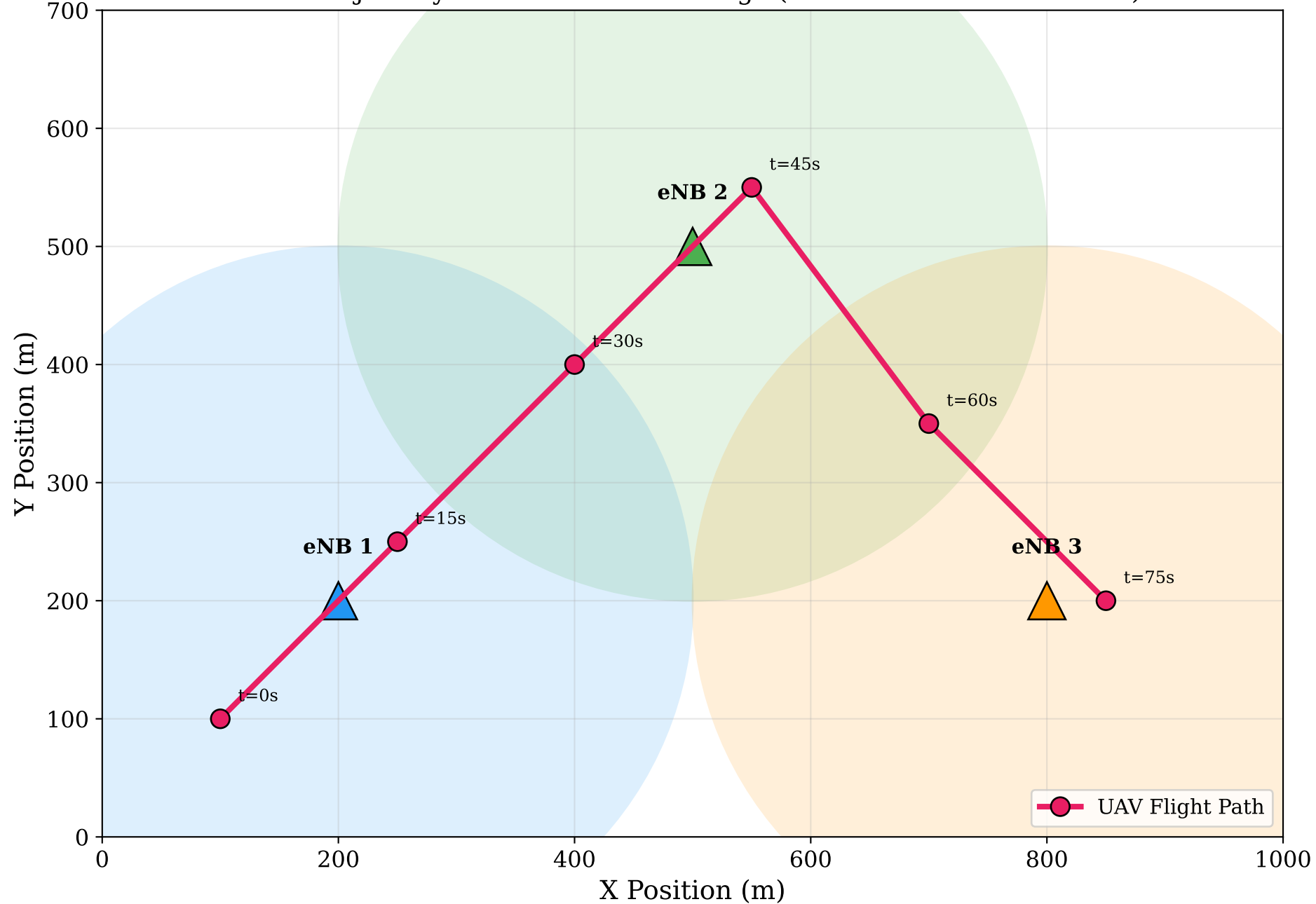
UAV Trajectory with LTE Cell Coverage (3GPP TR 36.777 Scenario)
