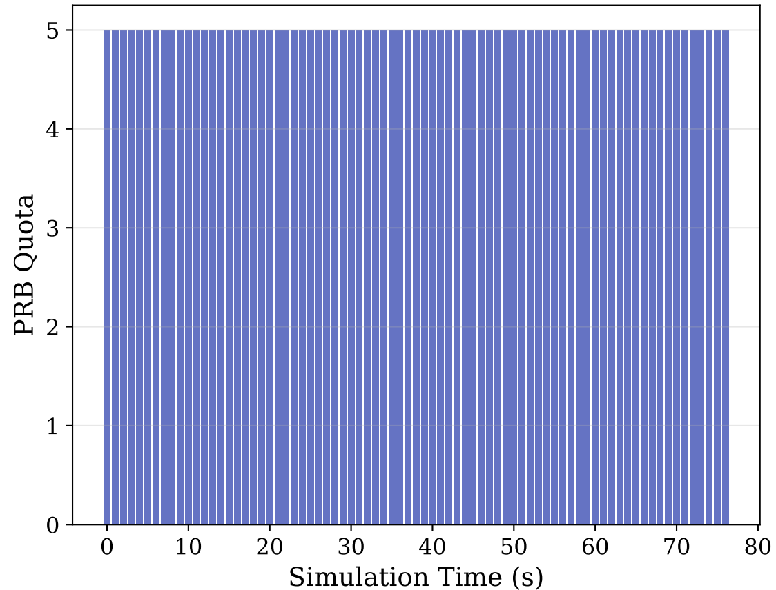
xApp PRB Resource Allocation
