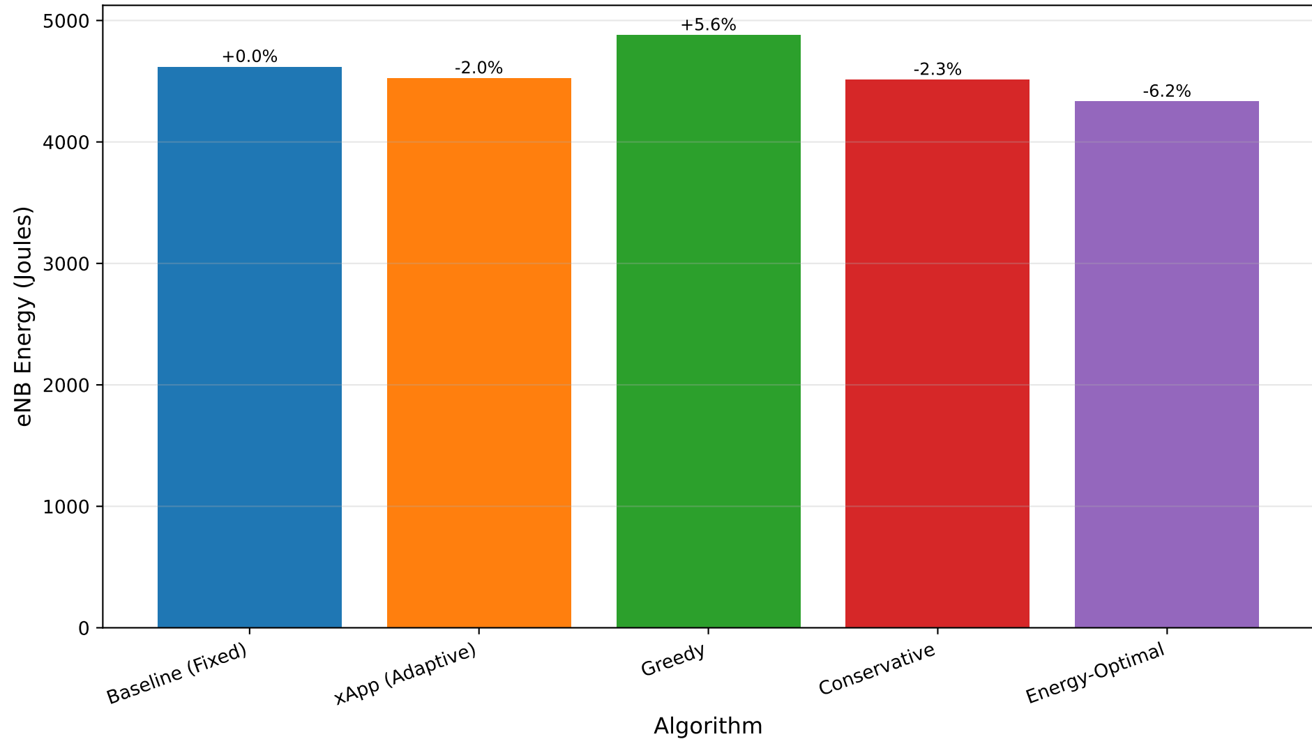
Network (eNB) Energy Consumption
