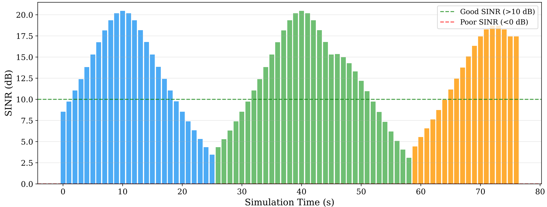
UAV SINR over Time (ns-3 LTE Simulation)
