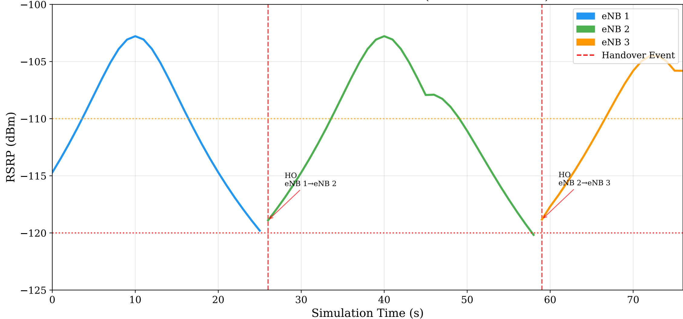
UAV RSRP Timeline with Cell Handovers (ns-3 LTE Simulation)
