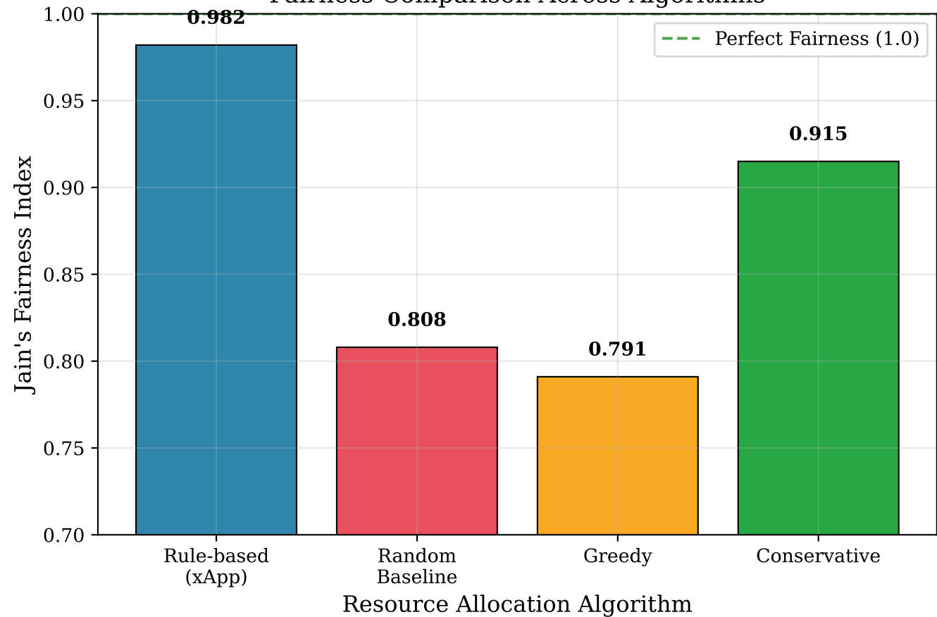
Fairness Comparison Across Algorithms
