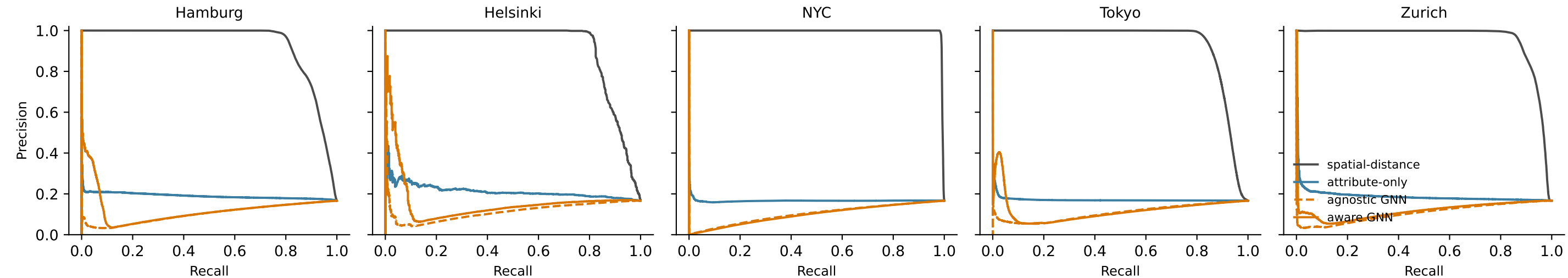
T3 cross-source matching: precision--recall, hard negatives
