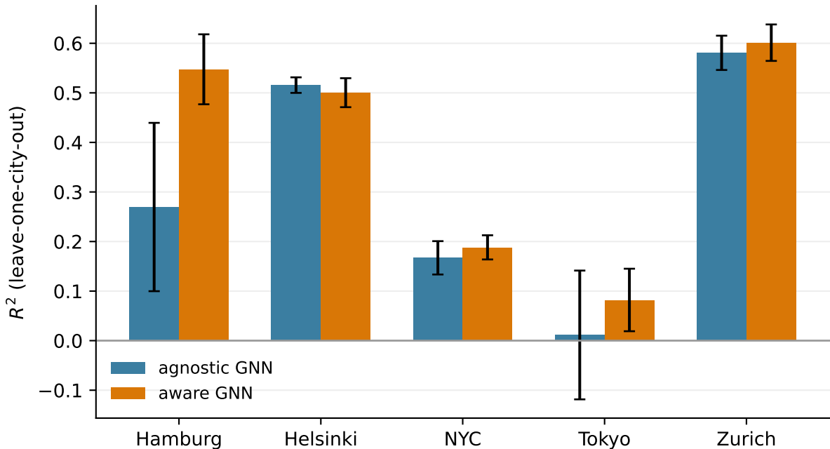
T1 height, cross-city transfer (mean over 10 seeds)
