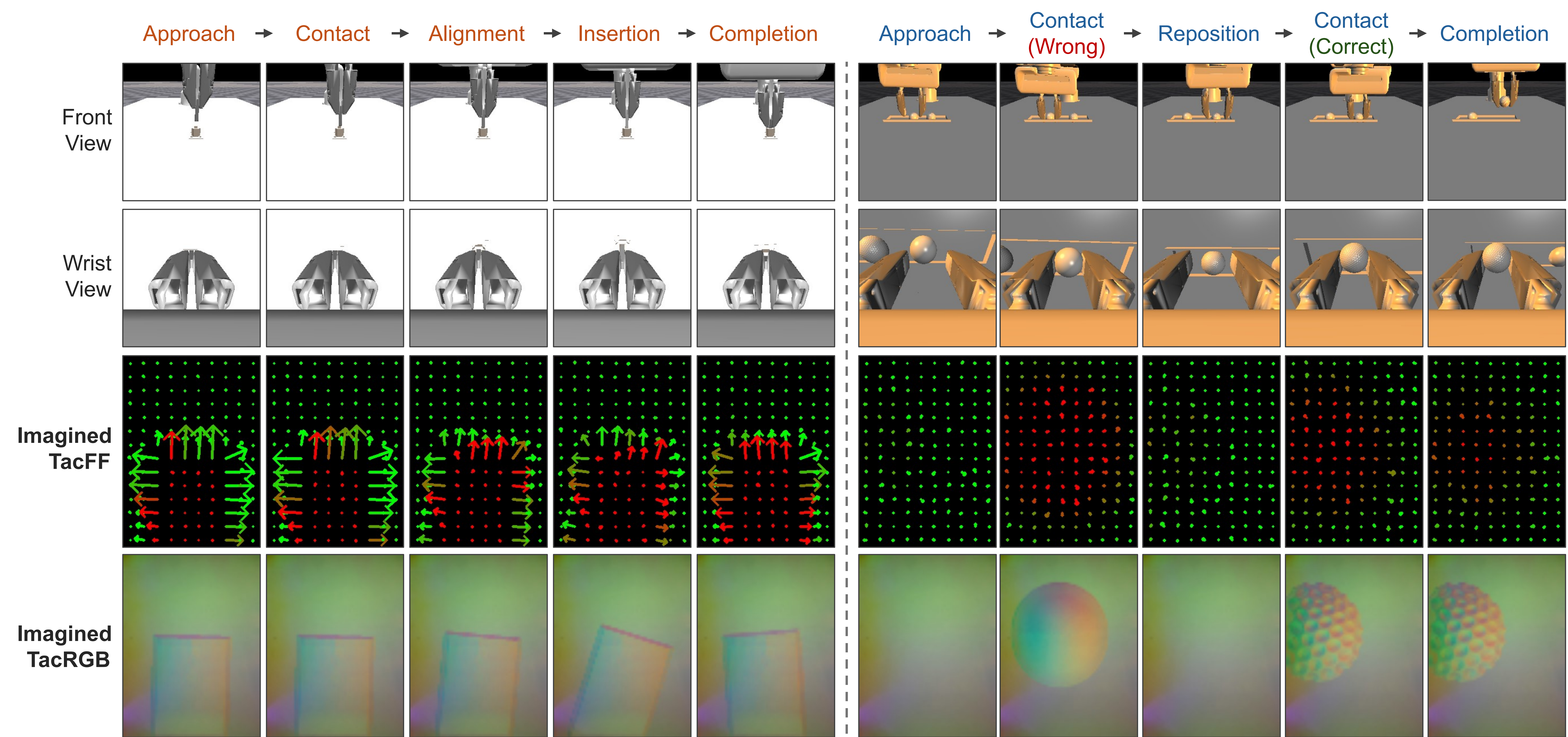
(a) Contact-Sensitive Task: Peg-in-Hole
