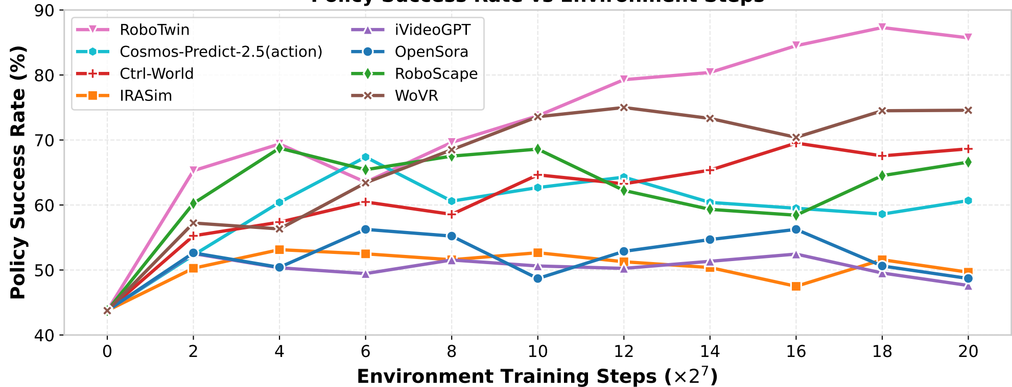
Policy Success Rate vs Environment Steps
