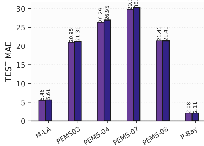
DPM baselines vs ZED (12→12)
