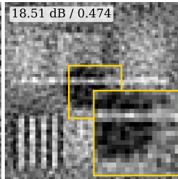
Tikhonov-GD
