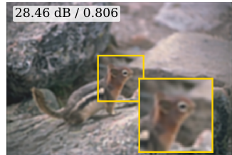
PnP-PGM
