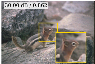
AdaptivePnP-PGM
