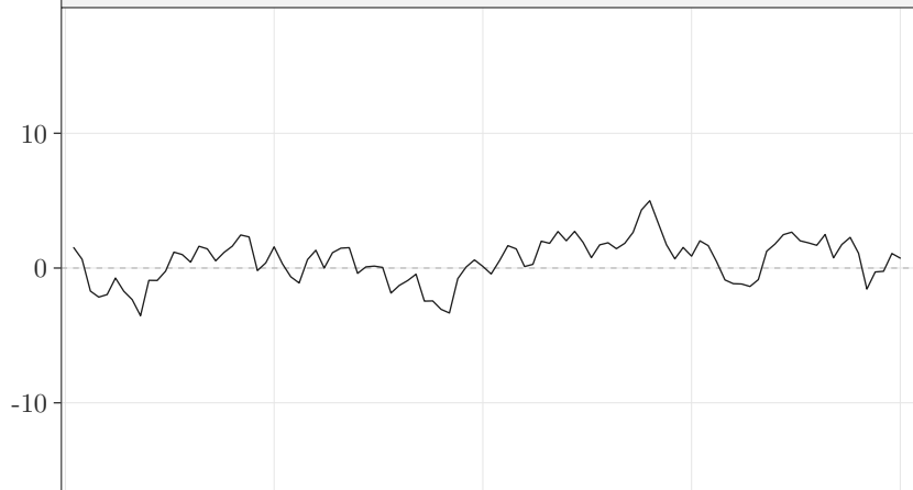
Stable VAR(1) \rho(\Phi_1) = 0.873
