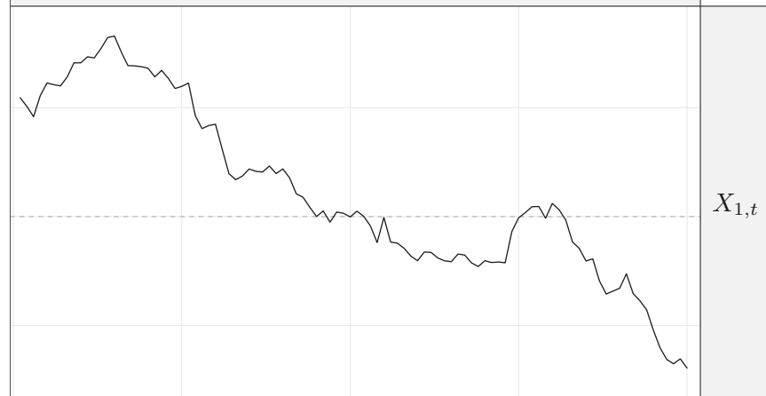
Unit-root boundary \rho(\Phi_1) = 1.000
