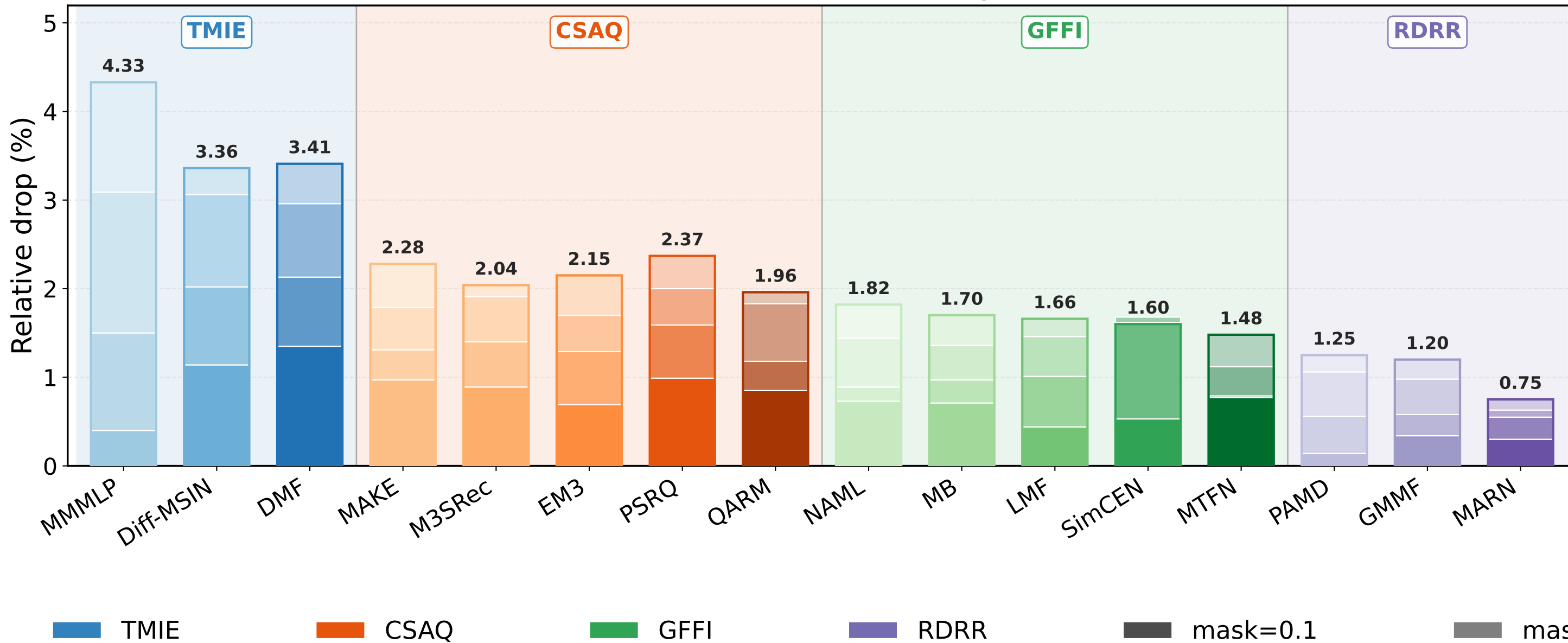
(a) Model-level cumulative degradation
