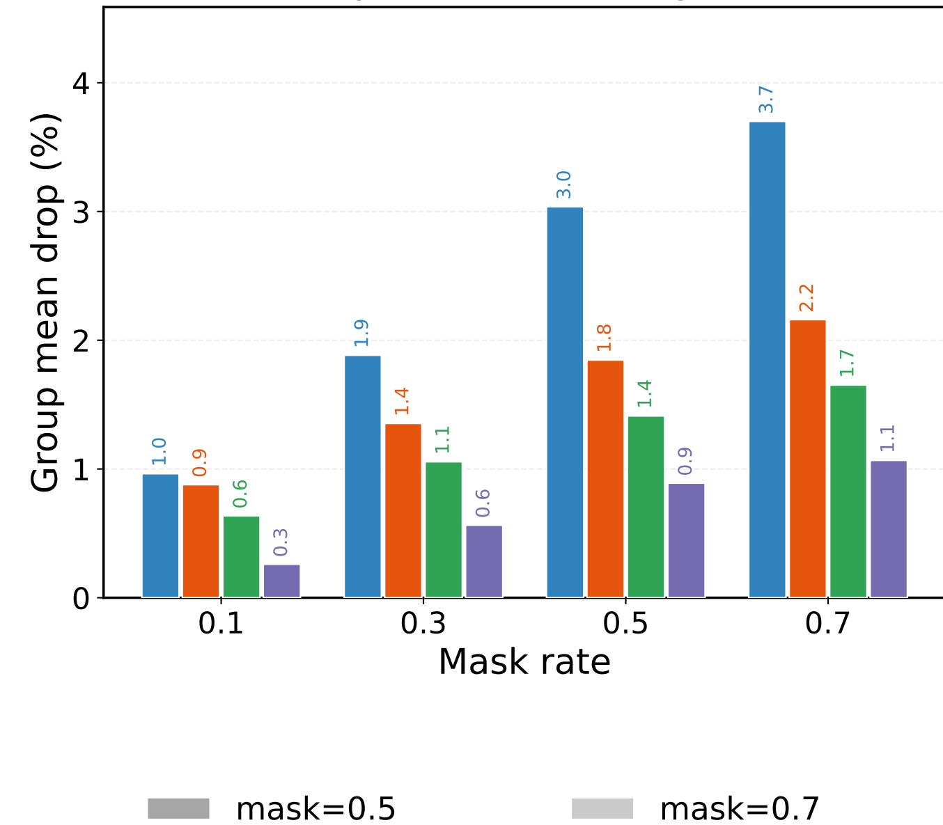
(b) Group-level mean degradation
