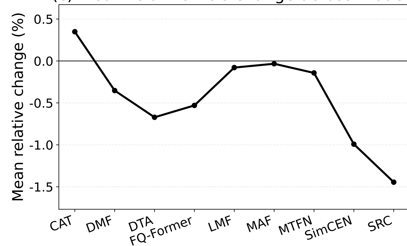
(c) Mean relative AUC change across models
