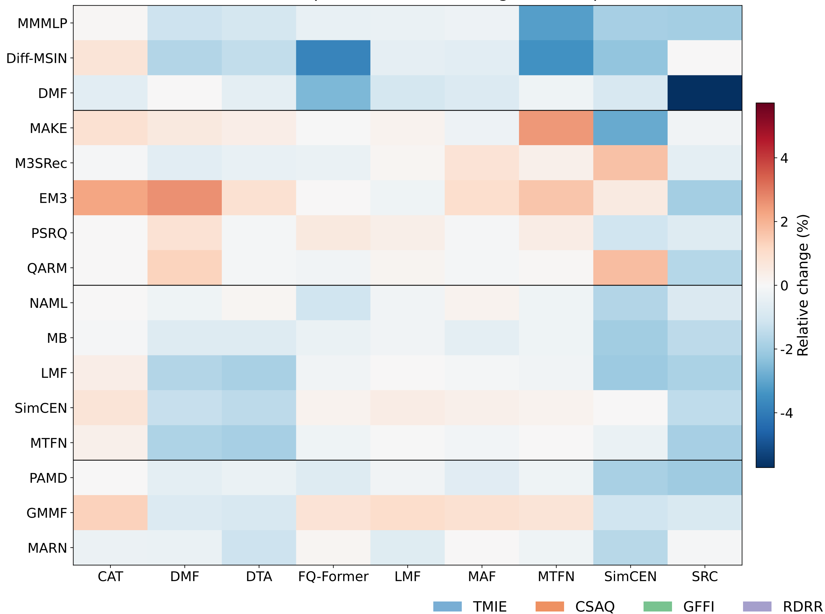
(a) Model-operator relative change heatmap
