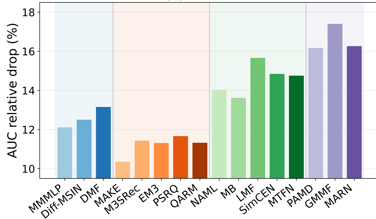
(b) zero-shot
