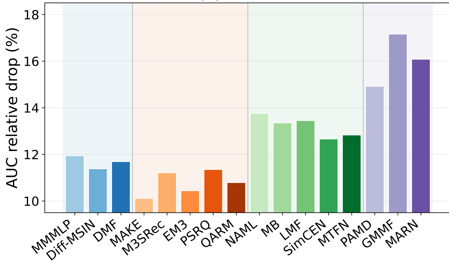
(a) few-shot
