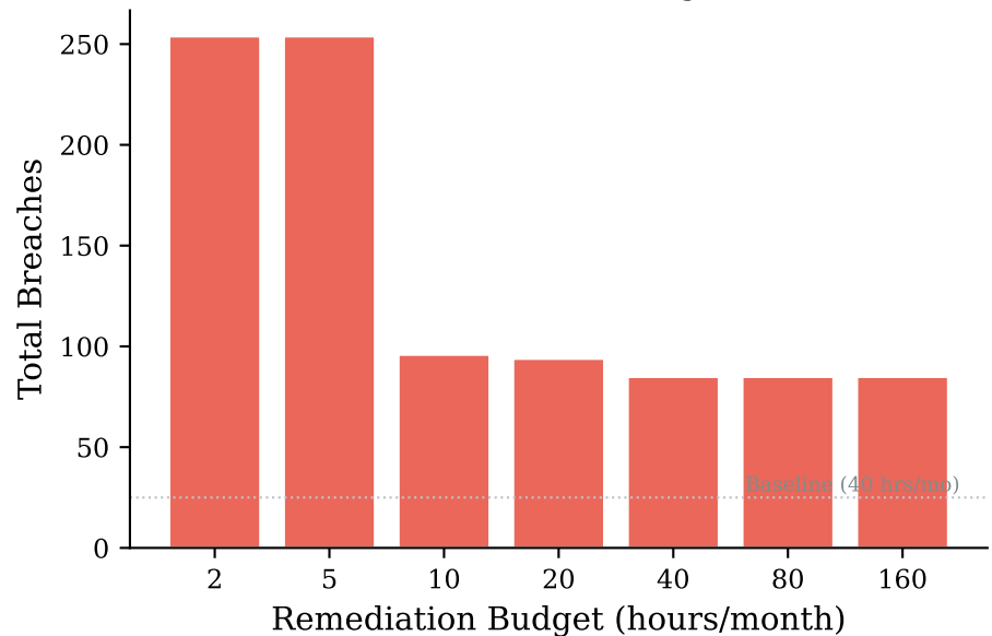
Breaches vs Budget
