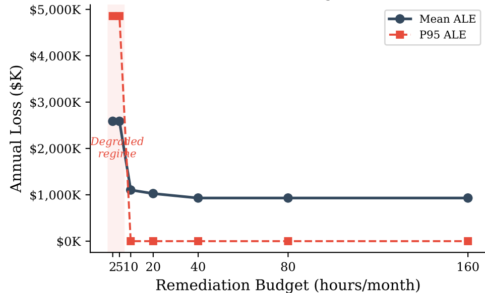
Loss vs Budget
