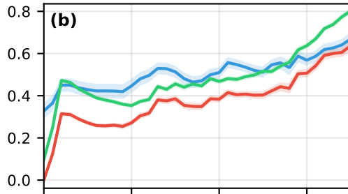
Qwen2.5-VL-3B
