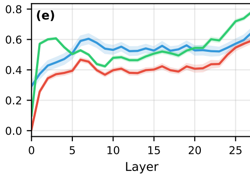
Qwen2.5-VL-7B
