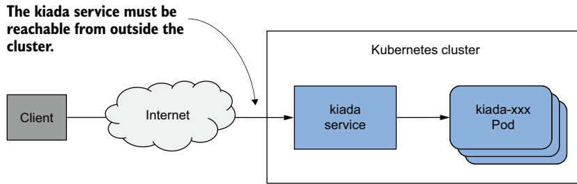
Figure 11.6 Exposing a service externally
