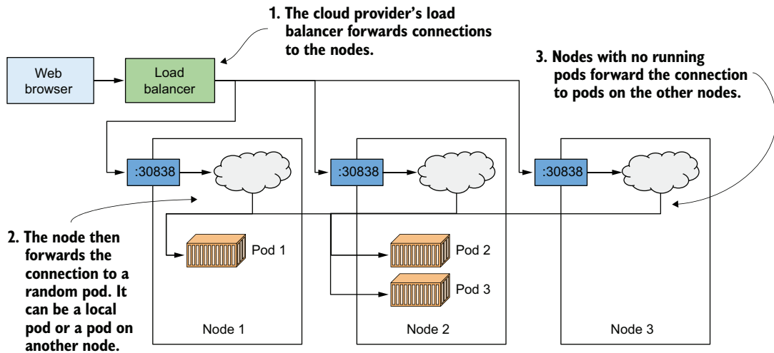
Figure 3.12 Load balancing across multiple pods backing the same service
