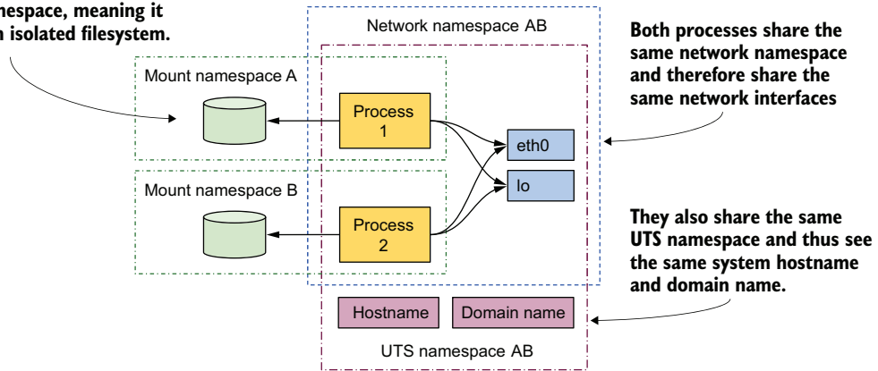
Figure 2.17 Each process is associated with multiple namespace types, some of which can be shared.
