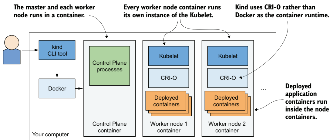
Figure 3.4 Running a multi-node Kubernetes cluster using kind
