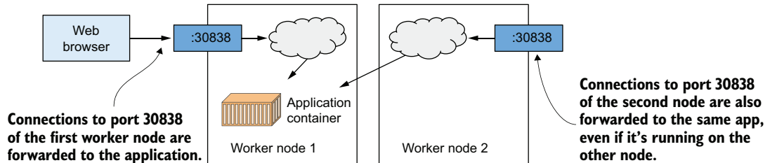
Figure 3.11 Connection routing through a service's node port
