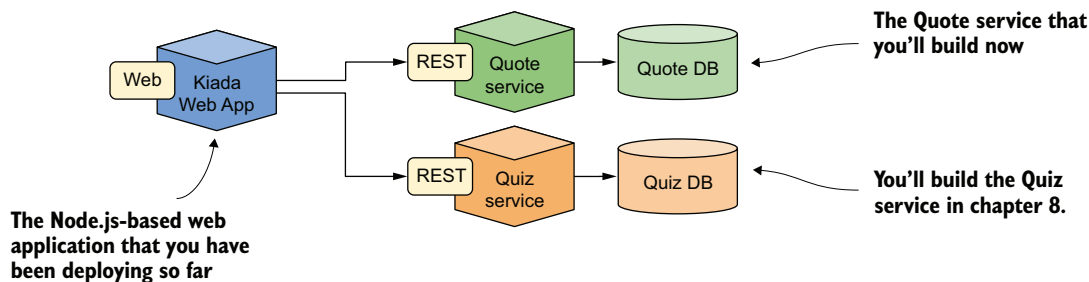
Figure 6.10 The Kubernetes in Action Demo Application Suite
