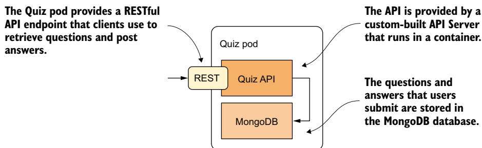
Figure 9.3 The Quiz API and the MongoDB database run in the same pod.
