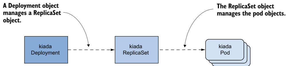
Figure 15.1 The relationship between Deployments, ReplicaSets and pods
