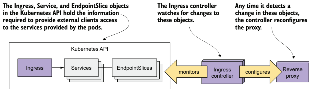
Figure 12.2 The role of an ingress controller
