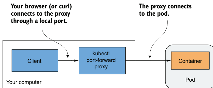
Figure 5.8 Connecting to a pod through the kubectl port-forward proxy
