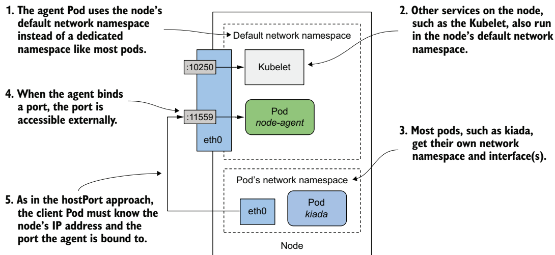
Figure 17.6 Exposing a daemon Pod by using the host node's network namespace
