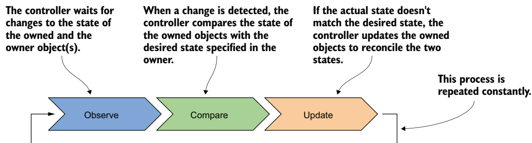
Figure 14.5 A controller's reconciliation control loop
