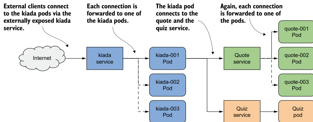
Figure 11.2 Exposing pods with Service objects
