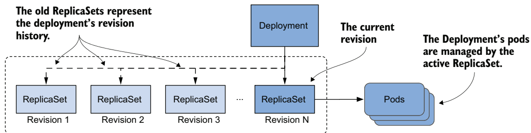
Figure 15.10 A Deployment's revision history
