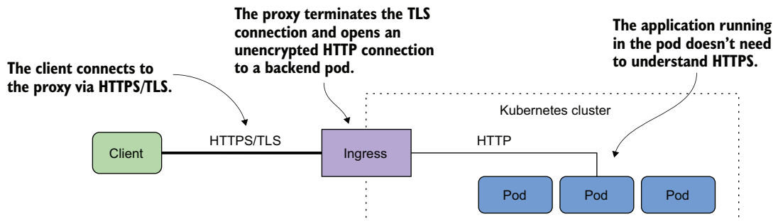
Figure 12.8 Securing connections to the Ingress using TLS
