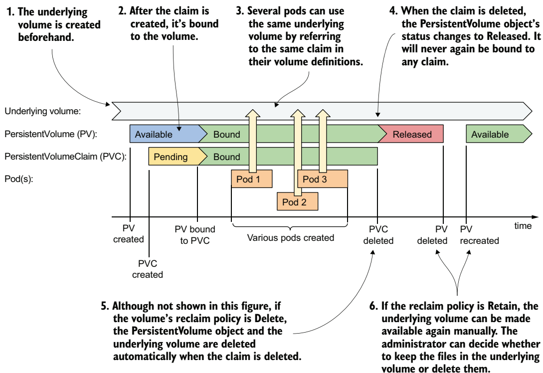
Figure 10.7 The life cycle of statically provisioned PersistentVolumes, claims, and the pods using them
