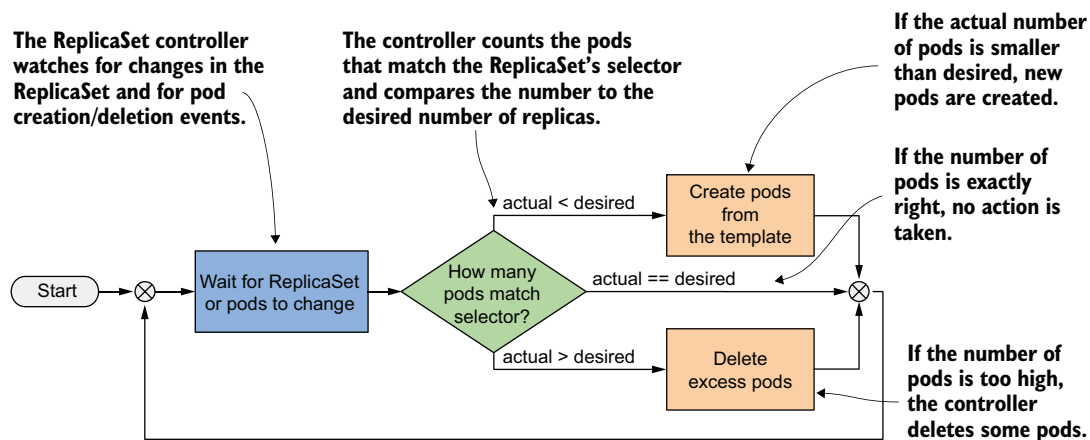
Figure 14.6 The ReplicaSet controller's reconciliation loop
