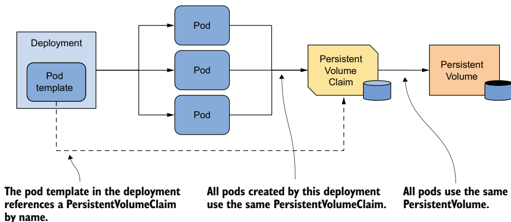
Figure 16.1 All pods from a Deployment use the same PersistentVolumeClaim and PersistentVolume.
