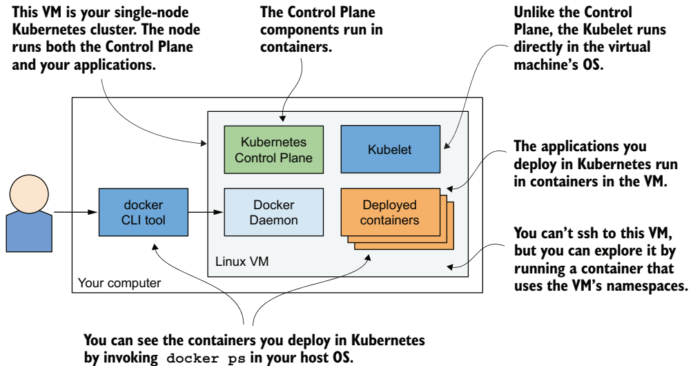
Figure 3.2 Kubernetes running in Docker Desktop
