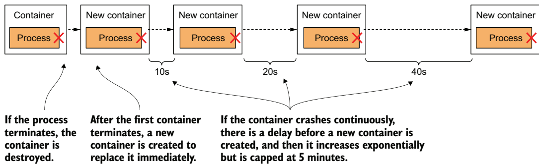
Figure 6.5 Exponential back-off between container restarts
