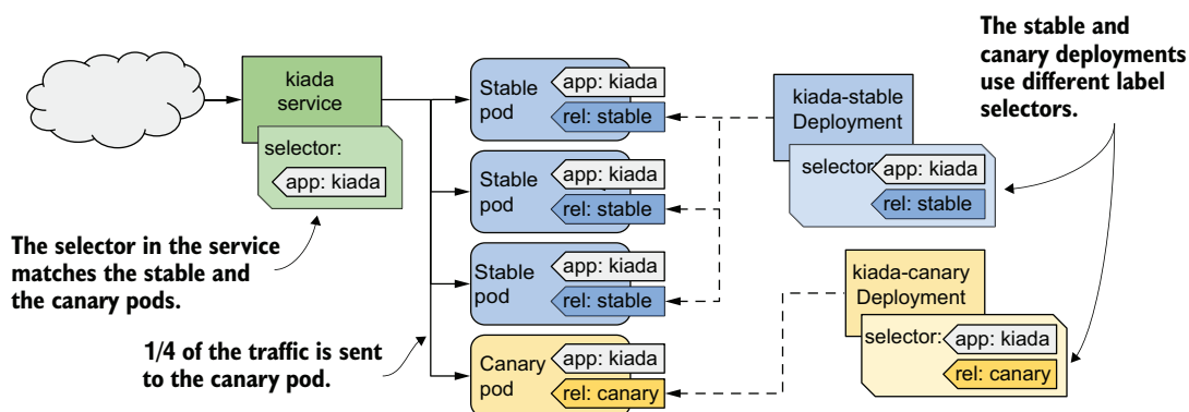
Figure 15.11 Implementing the Canary deployment strategy using two Deployments
