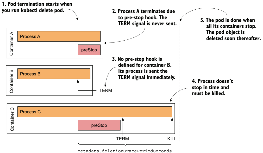
Figure 6.16 The termination sequence inside a pod
