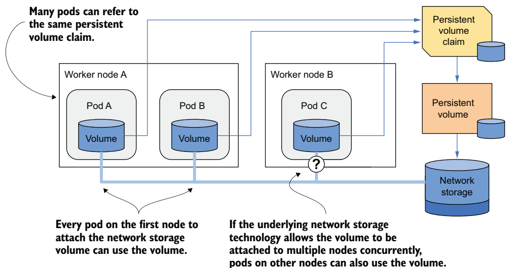
Figure 10.3 Using the same PersistentVolumeClaim in multiple pods
