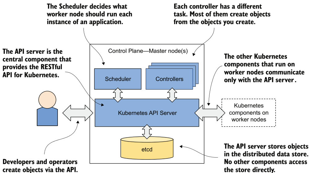
Figure 1.12 The components of the Kubernetes control plane
