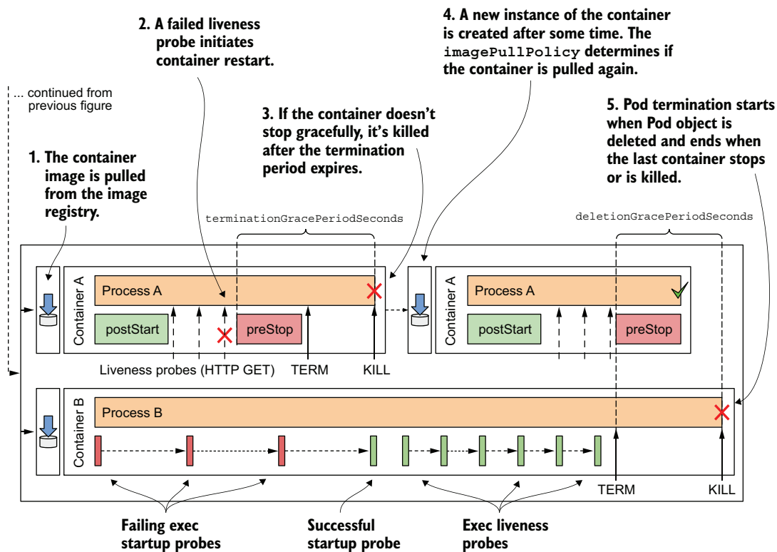
Figure 6.18 Complete overview of the pod's normal operation
