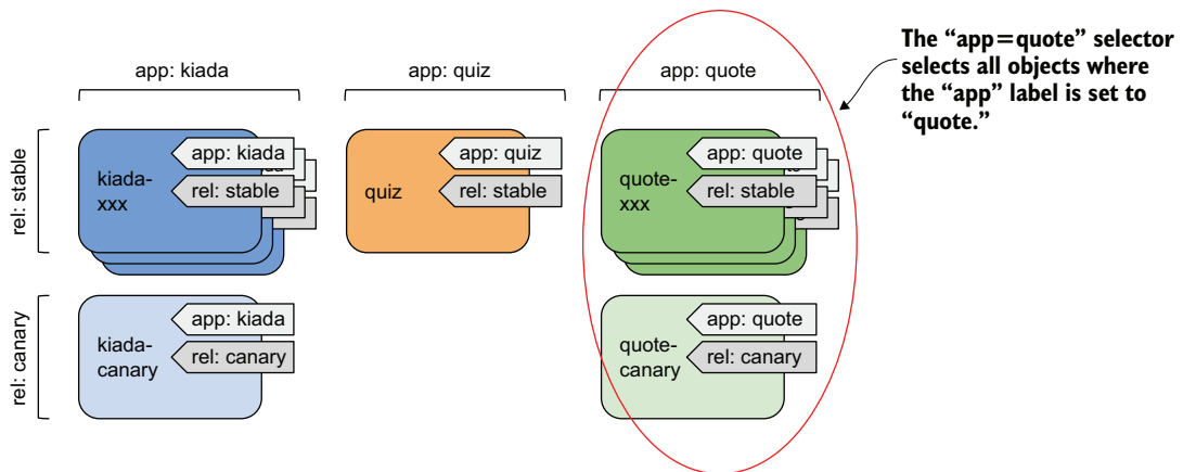
Figure 7.7 Selecting objects using an equality-based selector
