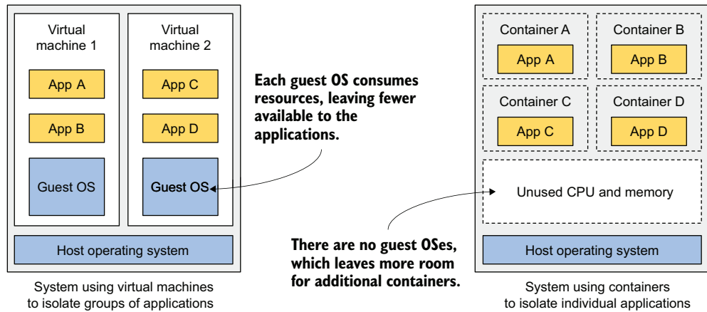
Figure 2.1 Running applications in VMs vs. containers
