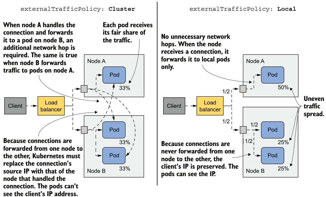
Figure 11.10 Understanding the two external traffic policies for NodePort and LoadBalancer services
