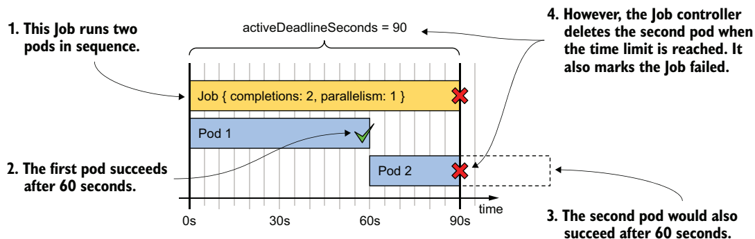
Figure 18.5 Setting a time limit for a Job
