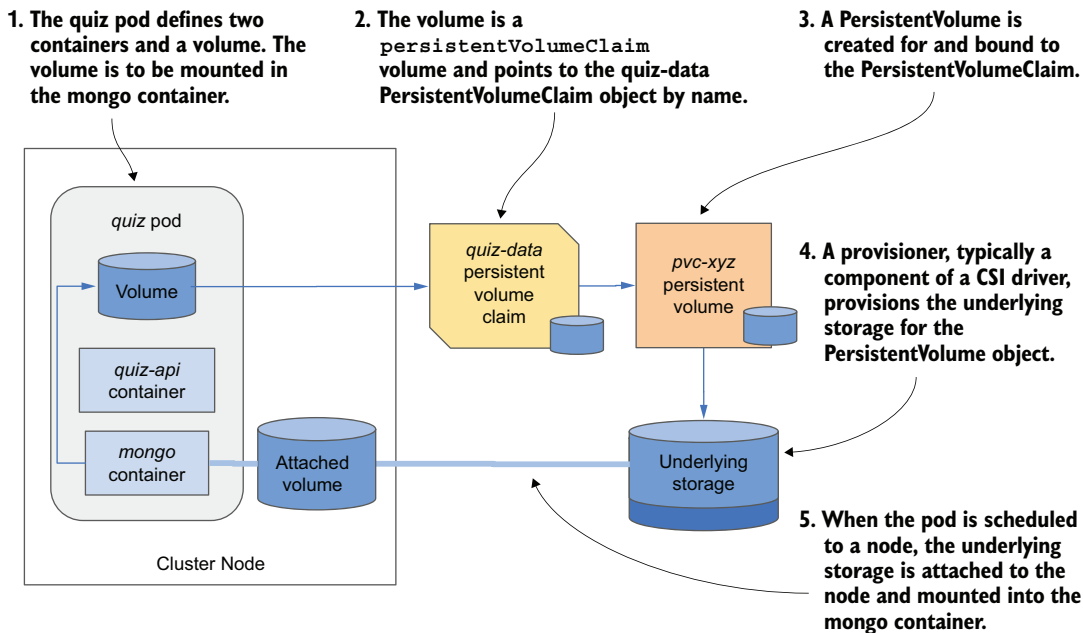
Figure 10.8 The quiz Pod and its PersistentVolume
