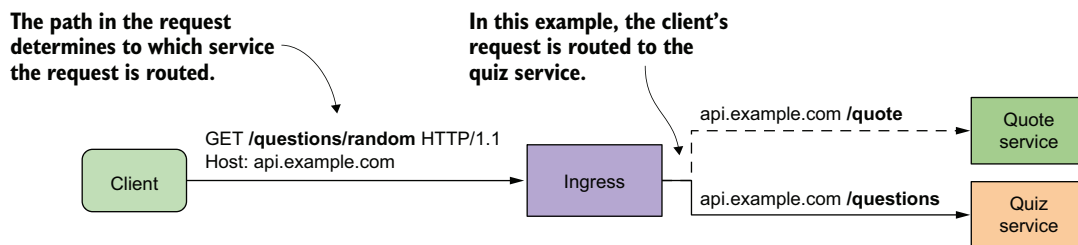
Figure 12.5 Path-based ingress traffic routing
