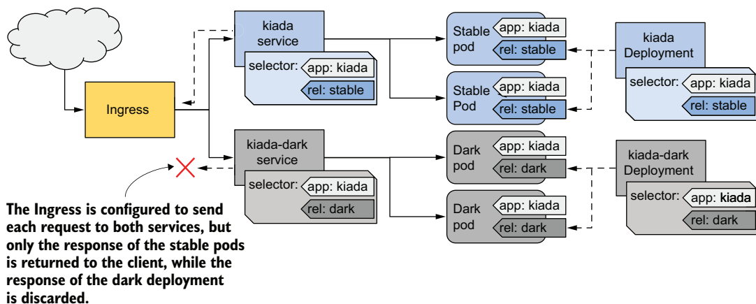
Figure 15.14 Implementing traffic shadowing
