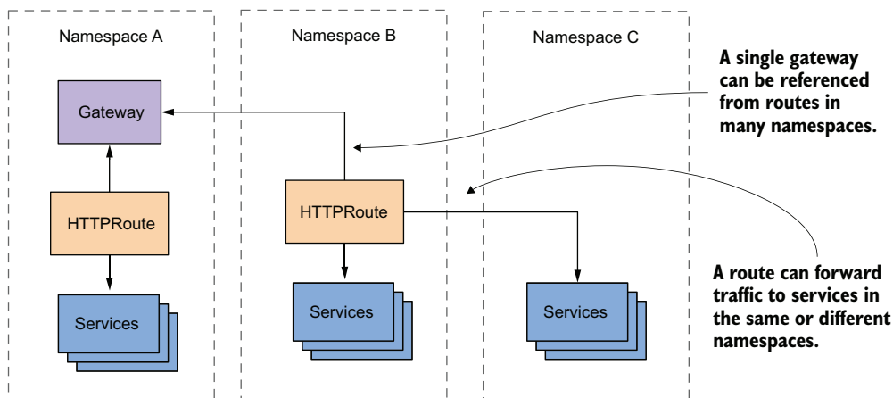
Figure 13.2 Using gateways and HTTPRoutes across namespaces
