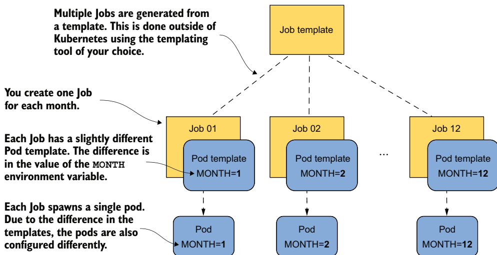
Figure 18.7 Creating similar Jobs from a template
