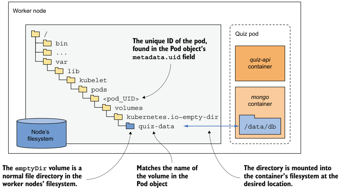
Figure 9.11 The emptyDir is a normal file directory in the node's filesystem mounted into the container.
