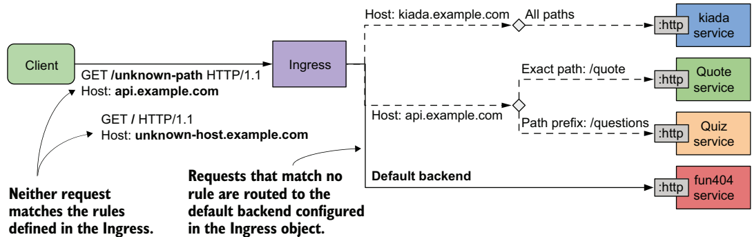
Figure 12.7 The default backend handles requests that match no ingress rule.
