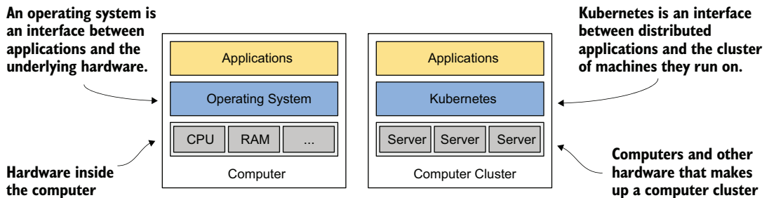
Figure 1.8 Kubernetes is to a computer cluster what an operating system is to a computer.
