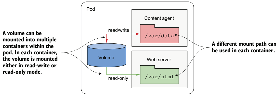
Figure 9.7 A volume can be mounted into more than one container.
