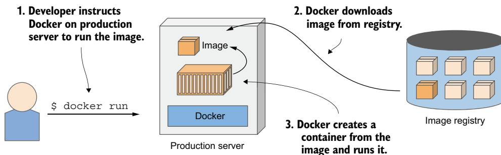
Figure 2.7 Running a container on a different computer
