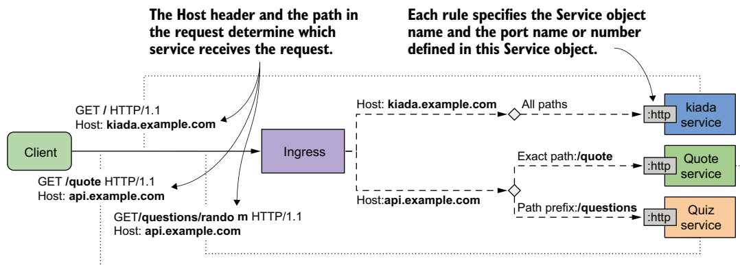
Figure 12.6 An Ingress object covering all services of the Kiada suite
