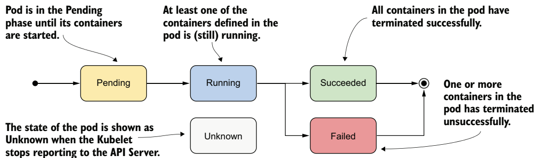
Figure 6.1 The phases of a Kubernetes Pod
