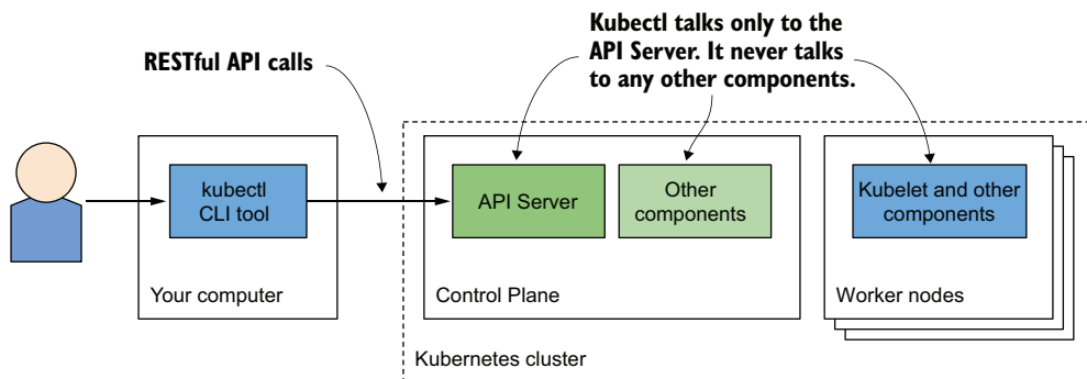
Figure 3.6 Interacting with a Kubernetes cluster
