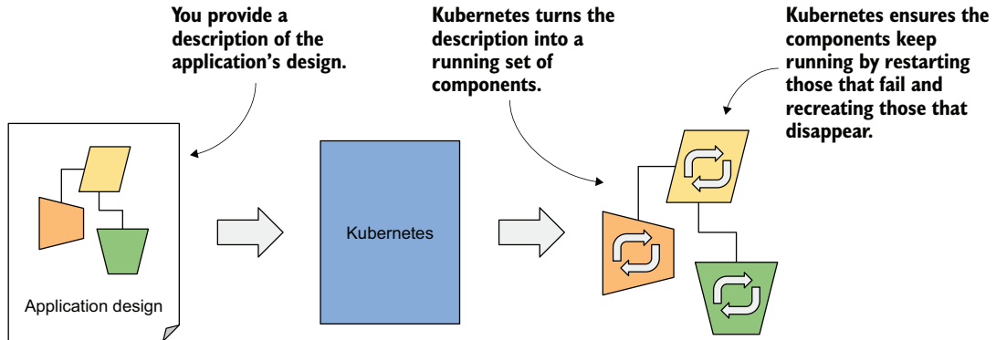
Figure 1.2 The declarative model of application deployment
