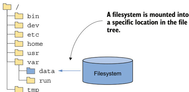
Figure 9.1 Mounting a filesystem into the file tree
