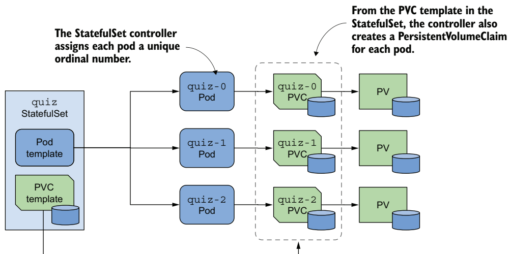
Figure 16.4 A StatefulSet, its pods, and PersistentVolumeClaims
