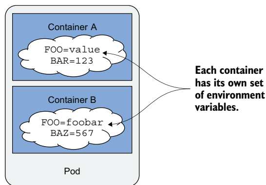
Figure 8.2 Environment variables are set per container.
