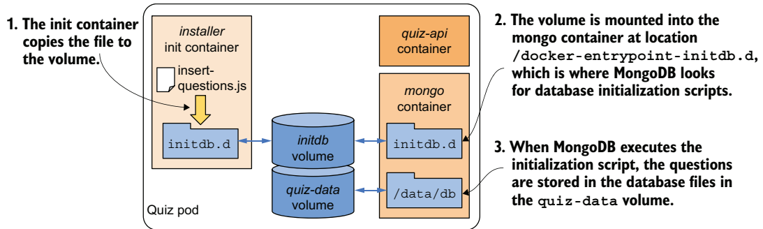
Figure 9.12 Using an init container to initialize an emptyDir volume
