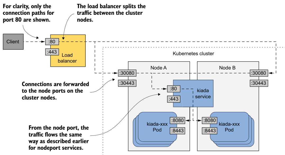
Figure 11.9 Exposing a LoadBalancer service
