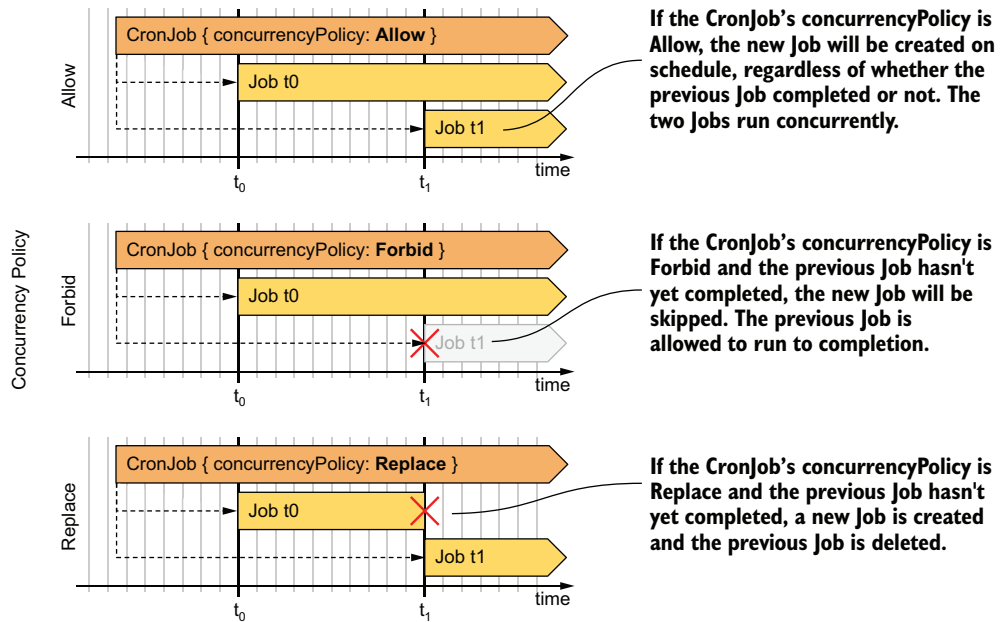
Figure 18.12 Comparing the behavior of the three CronJob concurrency policies
