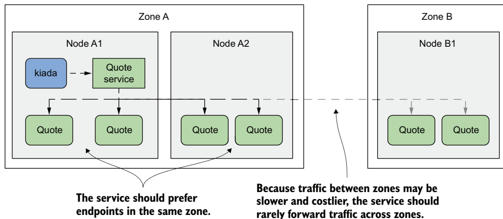
Figure 11.14 Routing serviced traffic across availability zones
