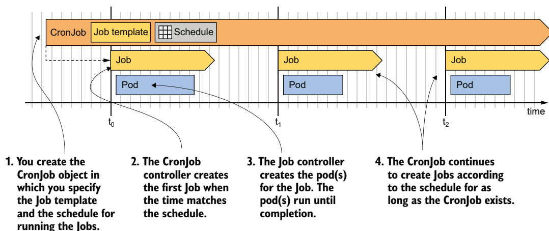
Figure 18.11 The operation of a CronJob
