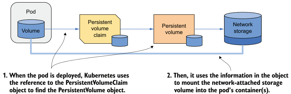
Figure 10.2 Mounting a PersistentVolume into the pod's container(s)
