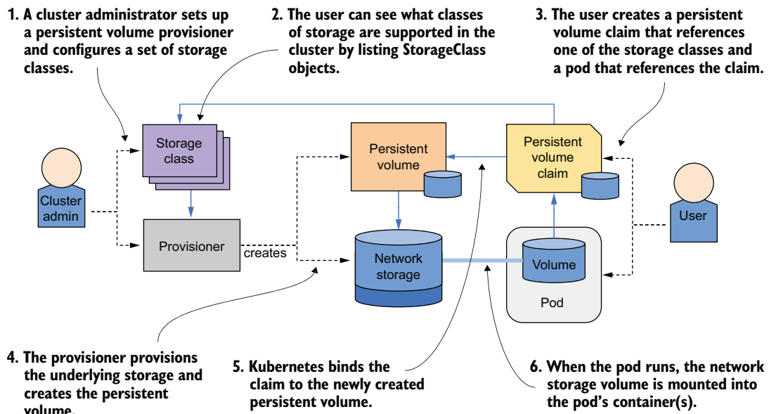
Figure 10.4 Dynamic provisioning of PersistentVolumes
