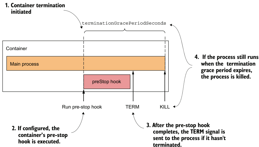
Figure 6.15 A container's termination sequence
