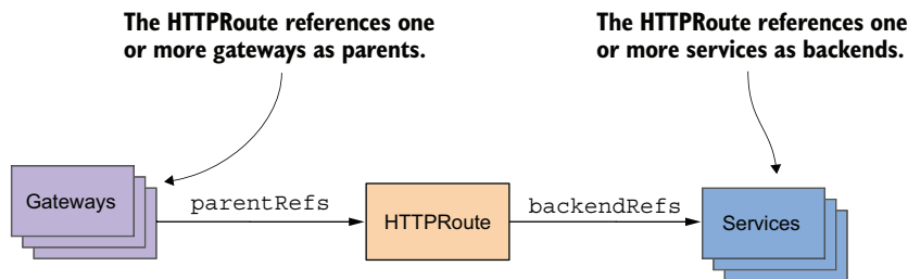
Figure 13.3 An HTTPRoute attaches one or more gateways to one or more services.
