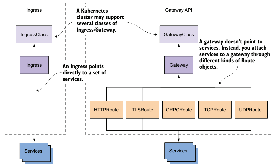
Figure 13.1 Comparing Ingress and Gateway API resources
