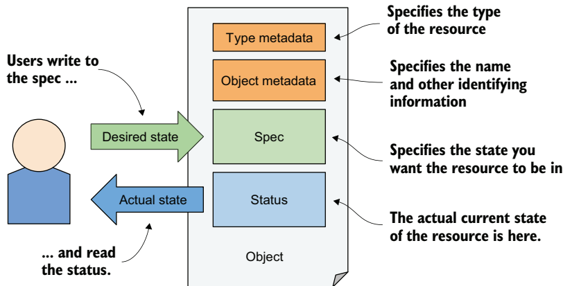
Figure 4.3 The main sections of a Kubernetes API object
