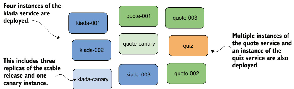
Figure 7.4 Unorganized pods of the Kiada application suite
