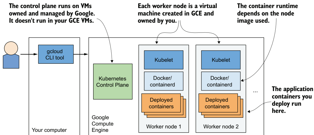
Figure 3.5 Your Kubernetes cluster in Google Kubernetes Engine
