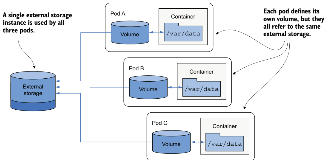
Figure 9.9 Using volumes to share data between pods
