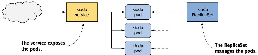
Figure 14.2 The relationship between services, ReplicaSets, and pods
