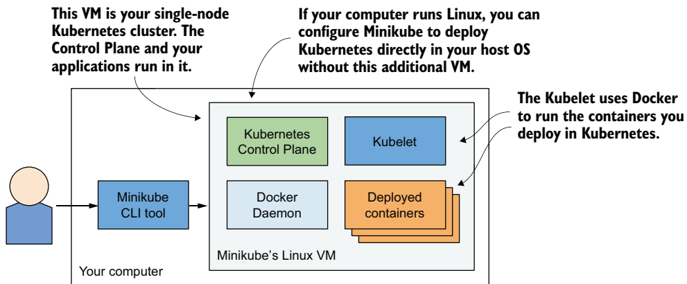
Figure 3.3 Running a single-node Kubernetes cluster using Minikube
