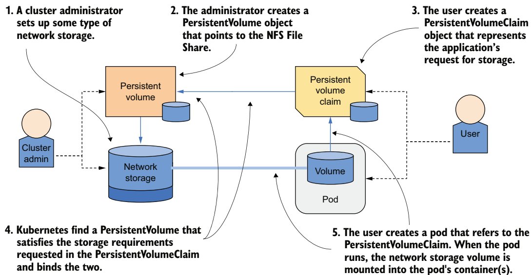
Figure 10.6 Static provisioning of PersistentVolumes
