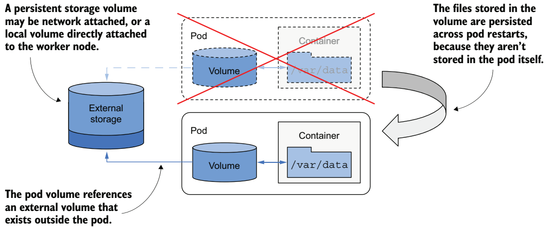
Figure 9.8 Pod volumes can also map to storage volumes that persist across pod restarts.
