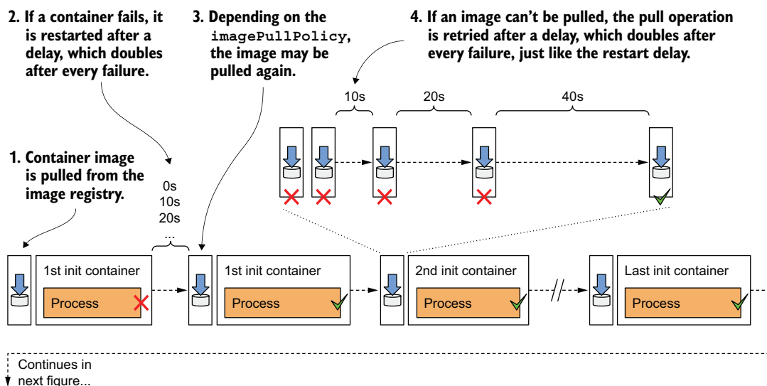
Figure 6.17 Complete overview of the pod's initialization stage
