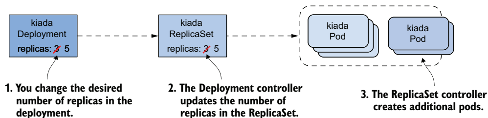
Figure 15.3 Scaling a Deployment
