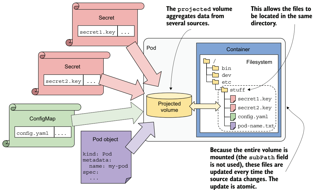
Figure 9.17 Using a projected volume with several sources
