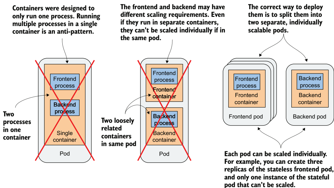
Figure 5.4 Splitting an application stack into pods
