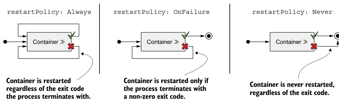
Figure 6.4 The pod’s restartPolicy determines whether its containers are restarted.
