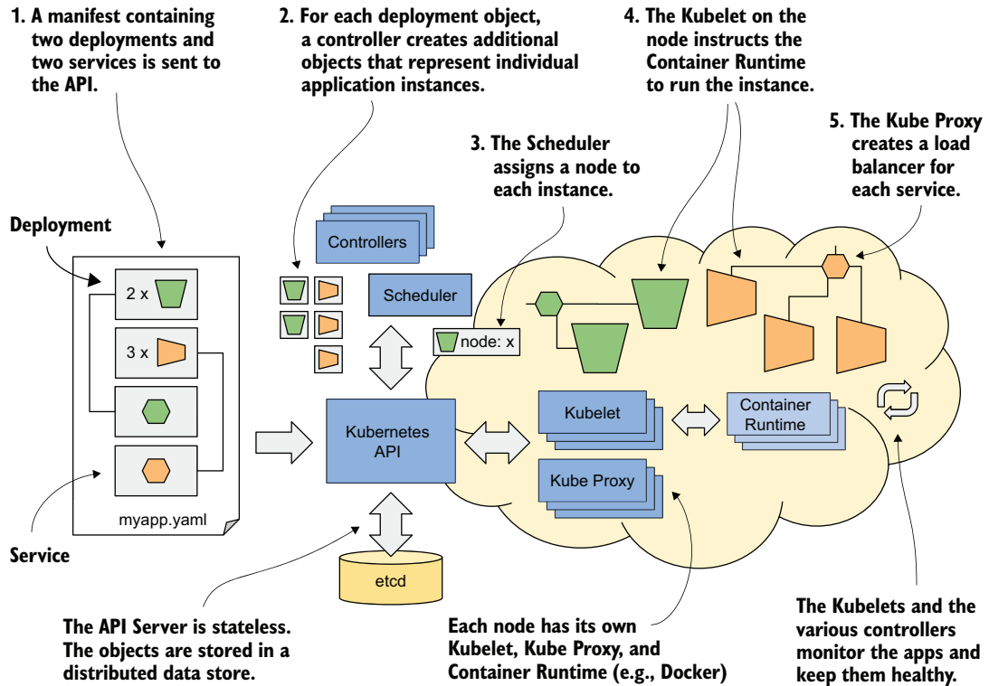
Figure 1.14 Deploying an application to Kubernetes
