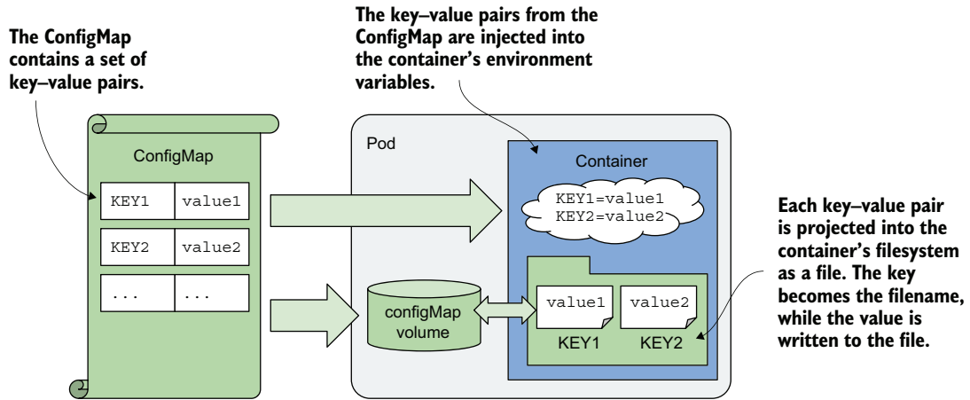
Figure 8.3 Pods use ConfigMaps through environment variables and ConfigMap volumes.
