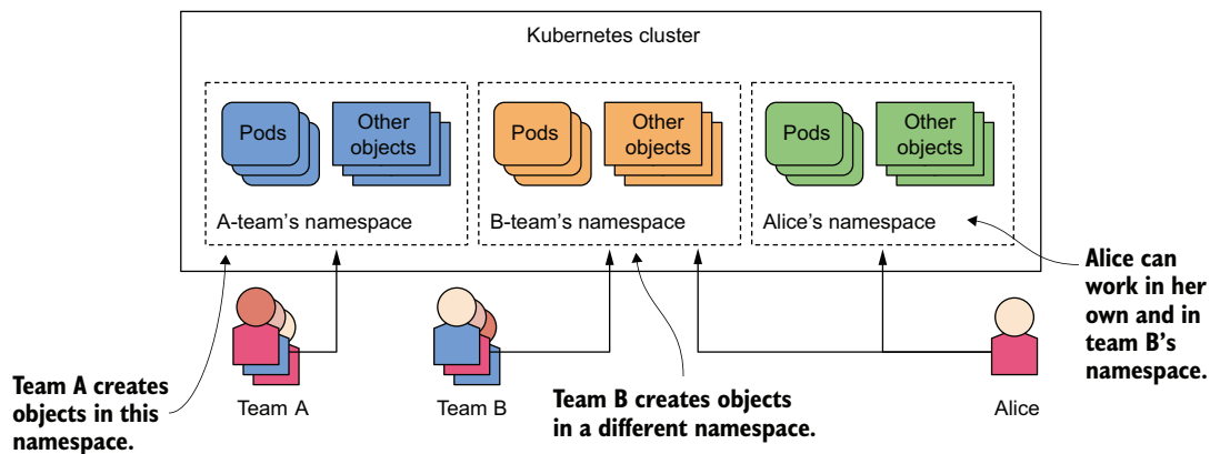
Figure 7.1 Splitting a physical cluster into several virtual clusters by utilizing Kubernetes Namespaces
