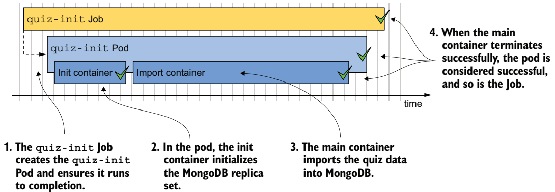
Figure 18.2 An overview of the quiz-init Job
