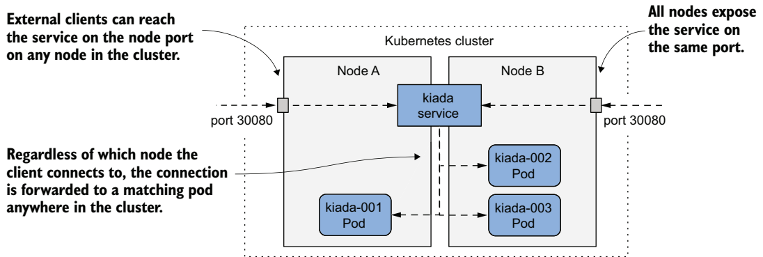
Figure 11.7 Exposing pods through a NodePort service
