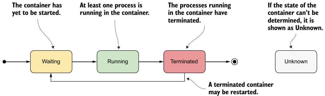
Figure 6.3 The possible states of a container
