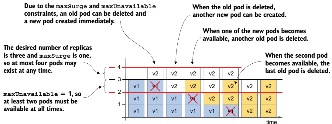
Figure 15.9 How pods are replaced when both maxSurge and maxUnavailable are 1
