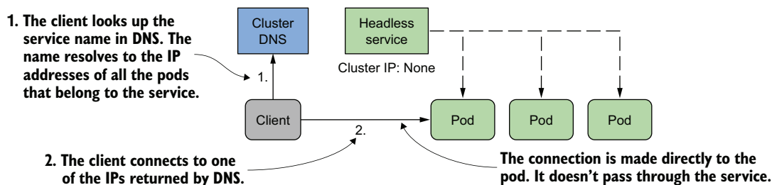
Figure 11.12 With headless services, clients connect directly to the pods.
