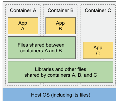
Figure 2.8 Containers can share image layers.
