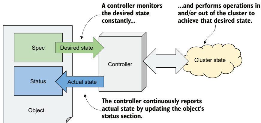
Figure 4.4 How a controller manages an object
