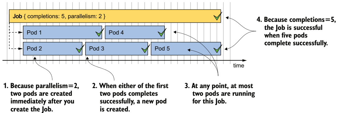
Figure 18.3 Running a parallel Job with completion = 5 and parallelism = 2
