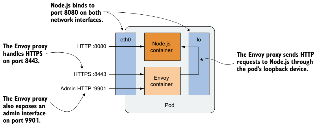
Figure 5.10 Detailed view of the pod's containers and network interfaces
