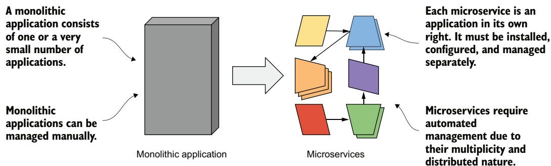
Figure 1.6 Comparing monolithic applications with microservices
