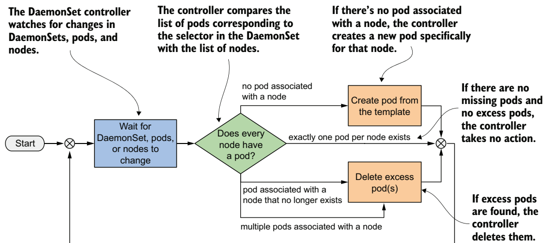
Figure 17.2 The DaemonSet controller's reconciliation loop
