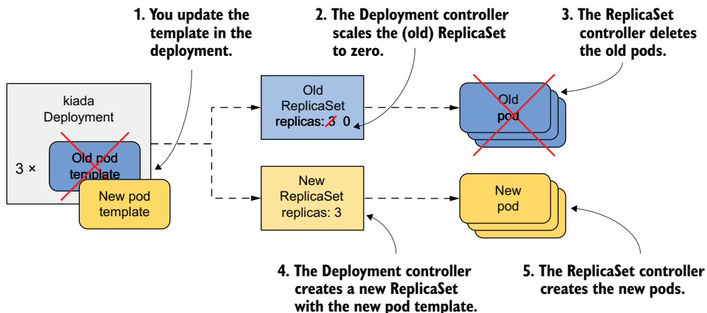
Figure 15.5 Updating a Deployment
