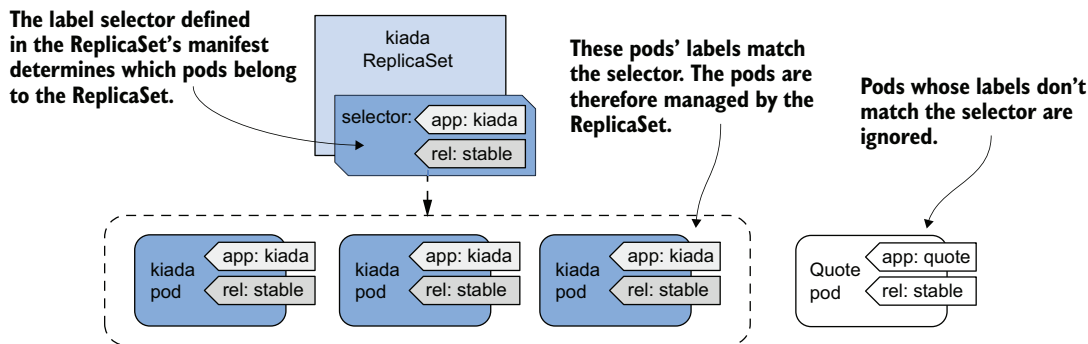
Figure 14.3 A ReplicaSet only cares about pods that match its label selector.
