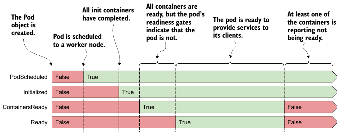
Figure 6.2 The transitions of the pod's conditions during its life cycle
