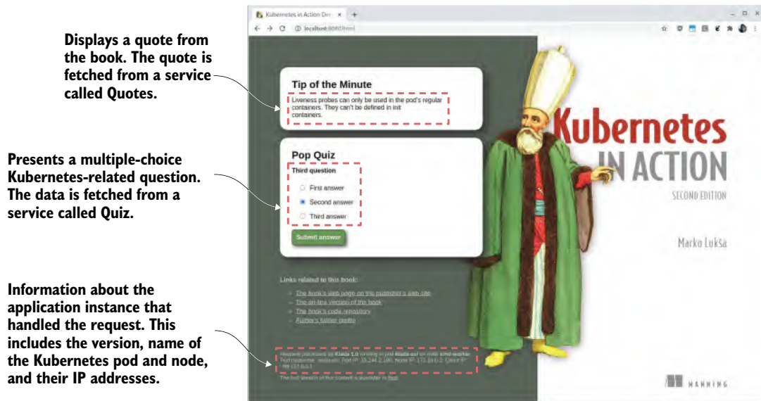
Figure 2.11 A screenshot of the Kubernetes in Action Demo Application (Kiada)
