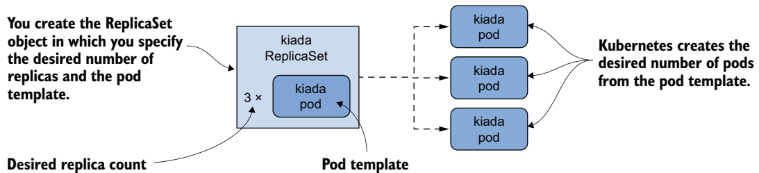
Figure 14.1 ReplicaSets in a nutshell
