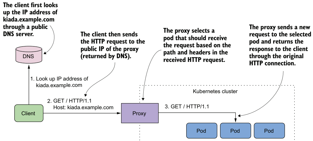
Figure 12.3 Accessing pods through an Ingress
