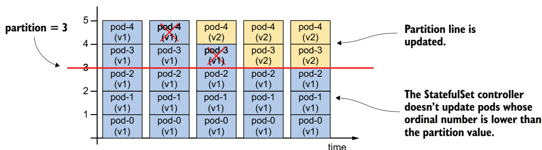
Figure 16.9 Partitioning a rolling update
