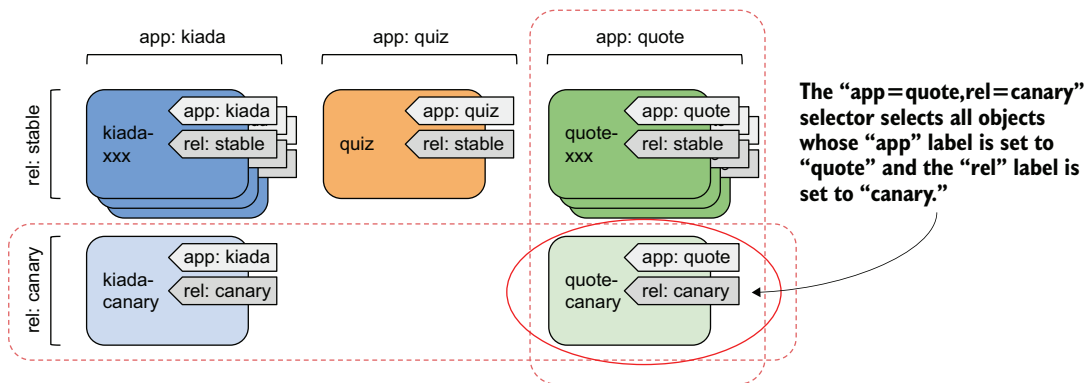
Figure 7.8 Combining two label selectors
