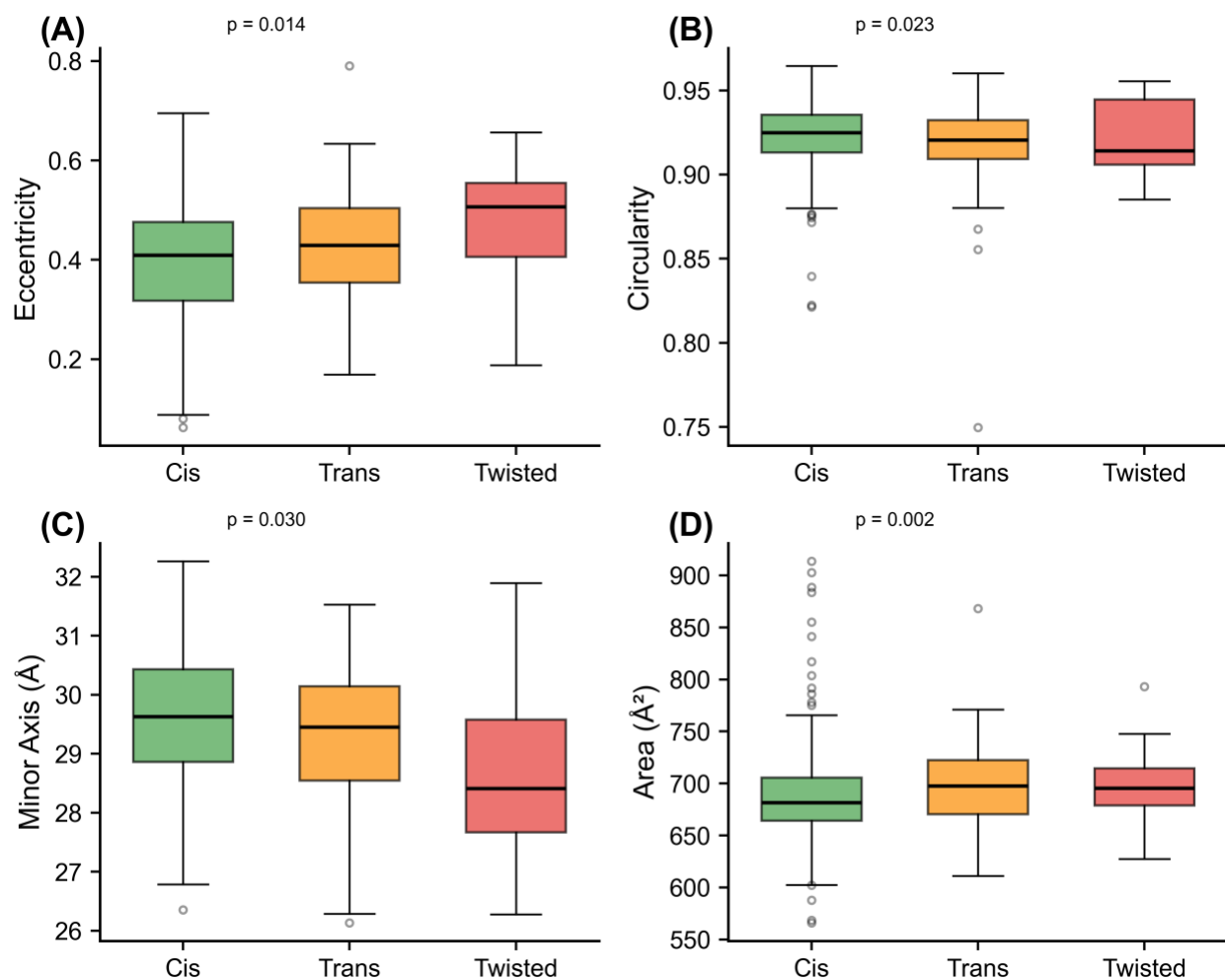
S4. Barrel geometry by chromophore configuration ( cis , trans , and twisted).
