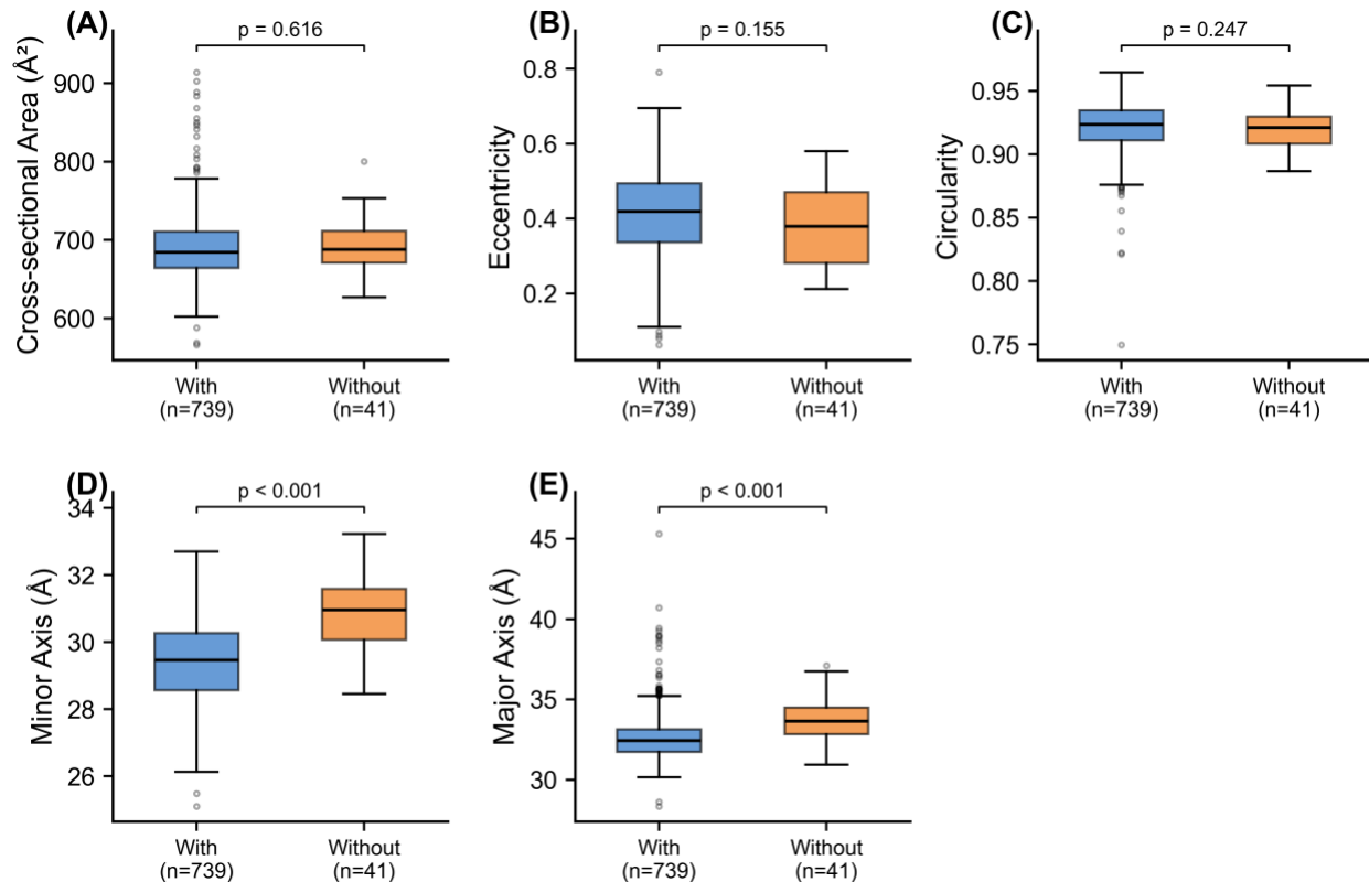
S1. Effect of chromophore maturation on barrel geometry within the canonical cohort ( n = 780 ). Boxplots compare structures with ( n = 739 , blue) and without ( n = 41 , orange) a validated mature chromophore. (A) Cross-sectional area, (B) eccentricity, and (C) circularity do not differ between the two groups. (D) Minor axis and (E) major axis are both narrower in chromophore-containing structures at the structure level ( p < 10^{-7} for both); these axis differences do not survive pseudoreplication collapse to one highest-resolution structure per unique protein (Table S2), reflecting the small number of unique chromophore-absent proteins ( n = 6 ) and the unbalanced group sizes. See main-text Chromophore Maturation section for interpretation.
