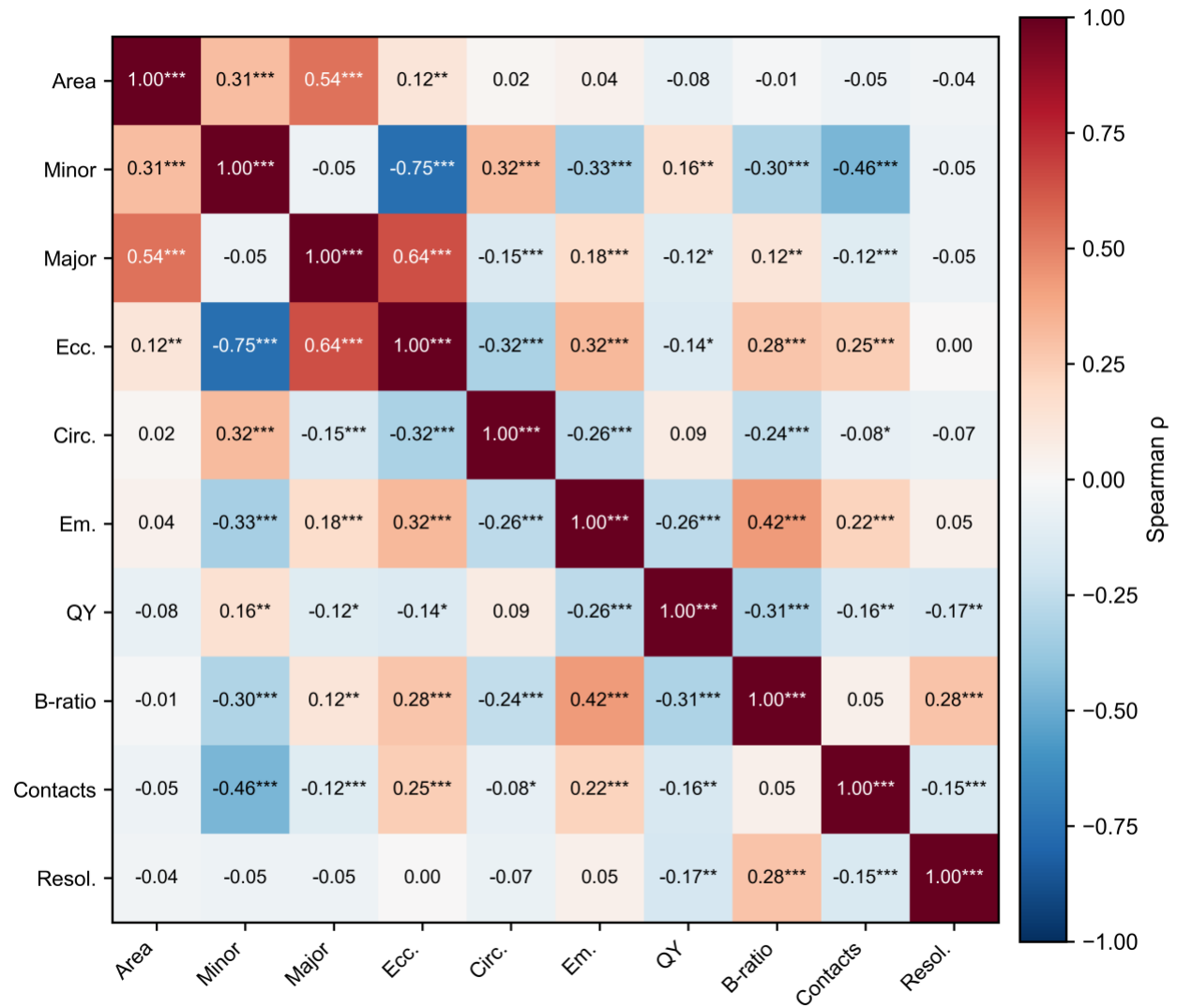
S7. Spearman correlation matrix for all variables. Asterisks indicate * p < 0.05, ** p < 0.01, *** p < 0.001.
