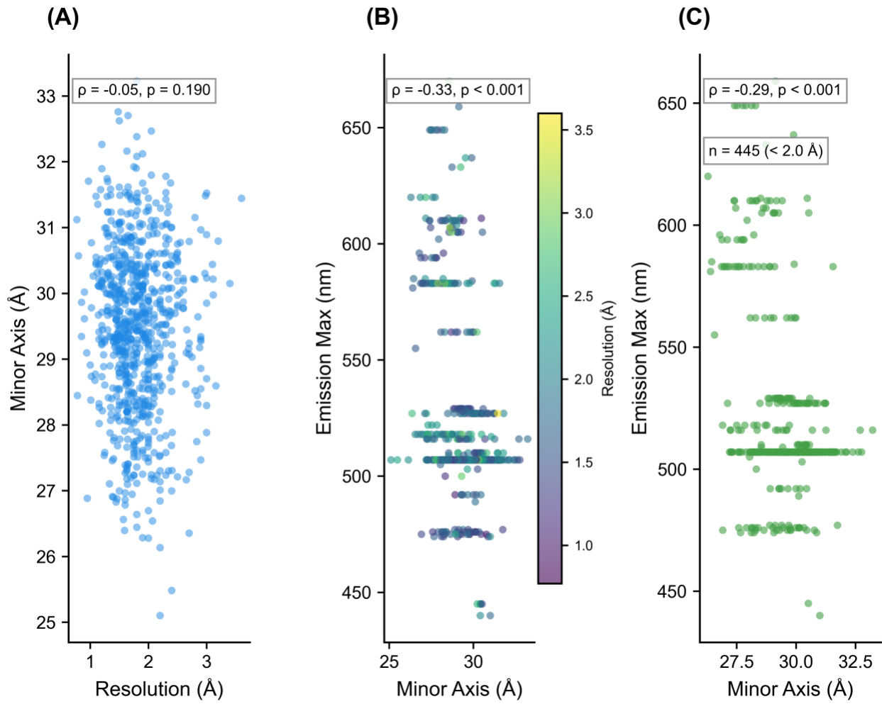
S5. Resolution control. (A) Resolution vs minor axis. (B) Emission vs minor axis colored by resolution. (C) High-resolution subset ( < 2.0 Å) only.
