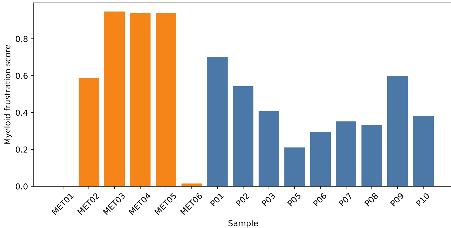
GSE154778 sample-level Myeloid frustration robustness
