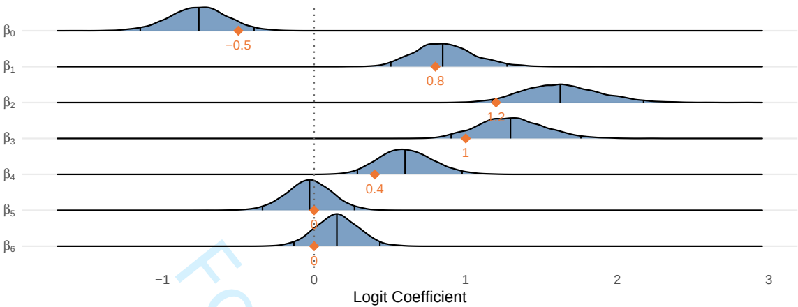
Ridgeline Plot of Posterior Distributions Posterior density with median & 95% HDI, Orange: True value.
