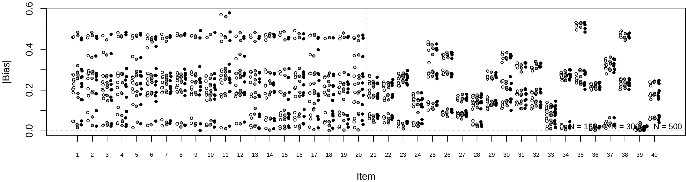
Simulation 3: |Bias| by item
