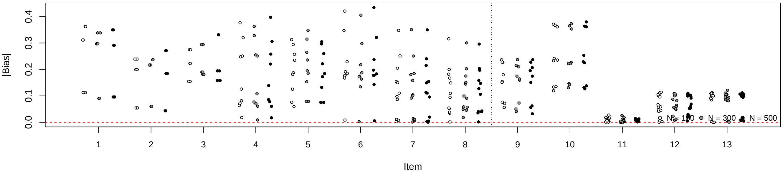
Simulation 2: |Bias| by item
