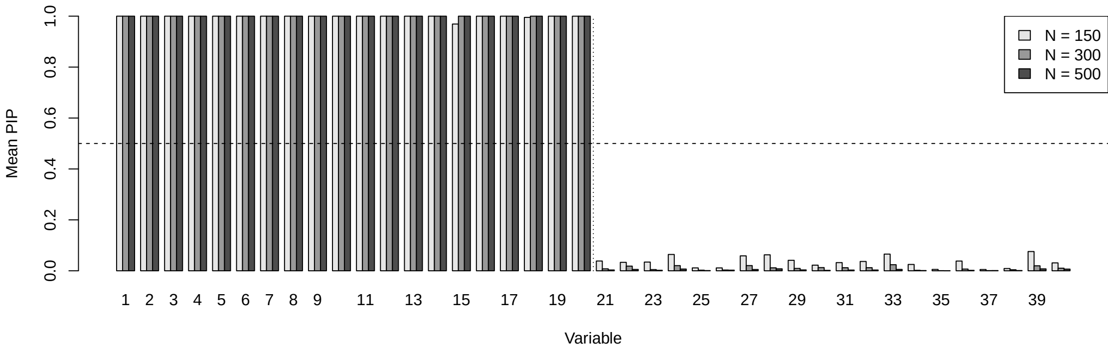
Simulation 3: Posterior Inclusion Probabilities (Items)
