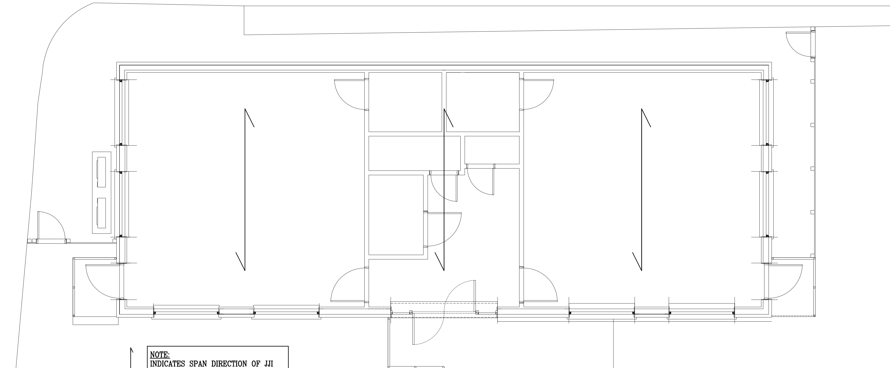
ROOF PLAN SCALE 1:50
