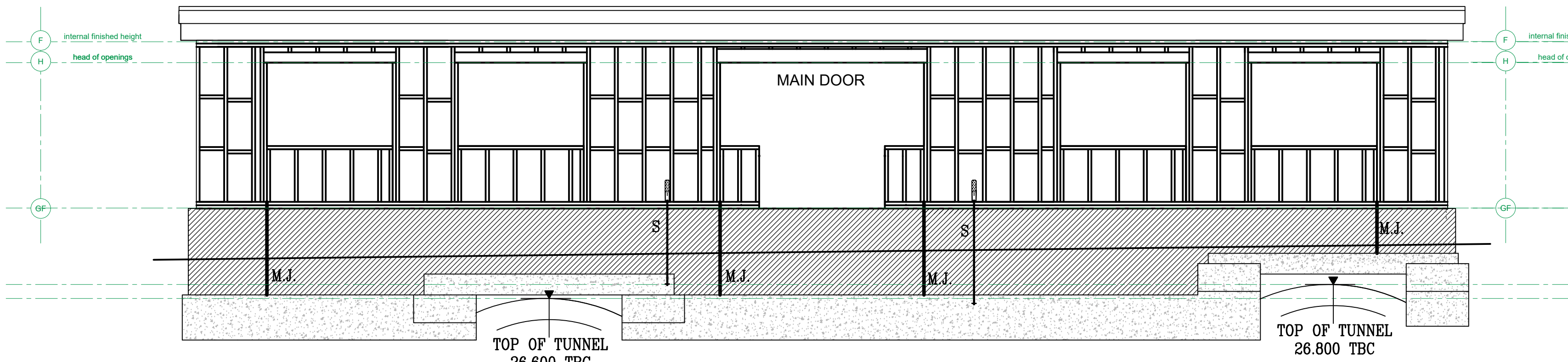
ELEVATION ON GRIDLINE C SCALE 1:50
