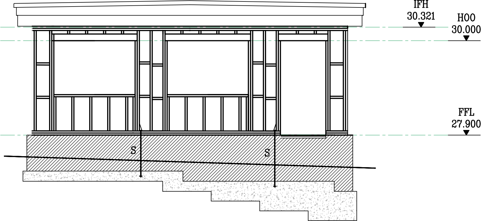
ELEVATION ON GRIDLINE 1 SCALE 1:50
