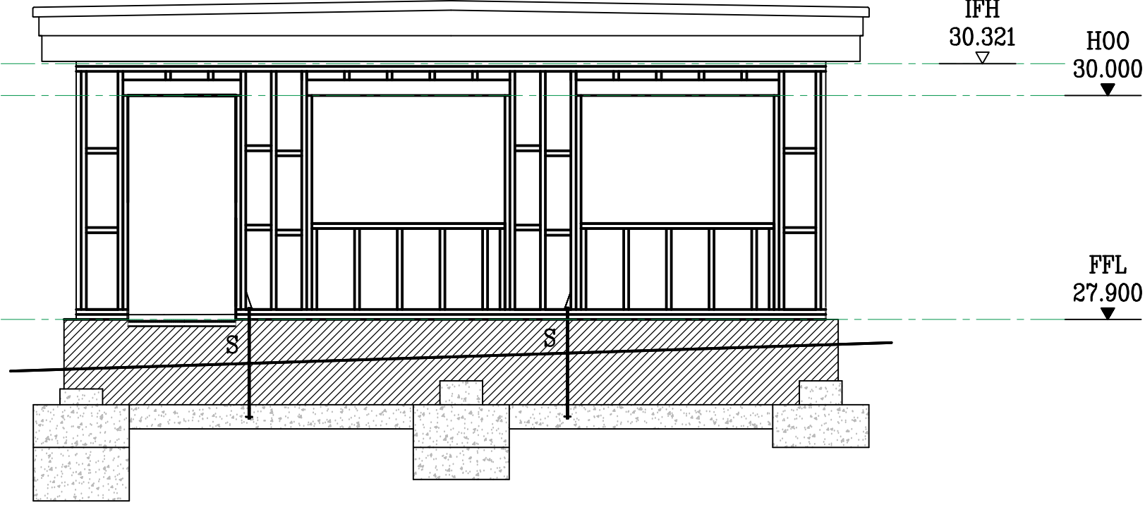
ELEVATION ON GRIDLINE 5 SCALE 1:50
