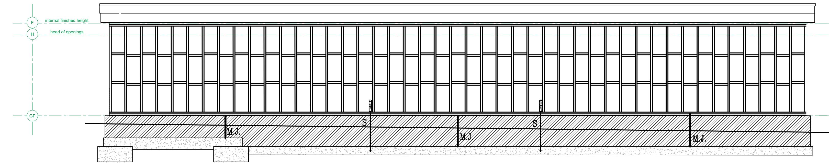
ELEVATION ON GRIDLINE A SCALE 1:50
