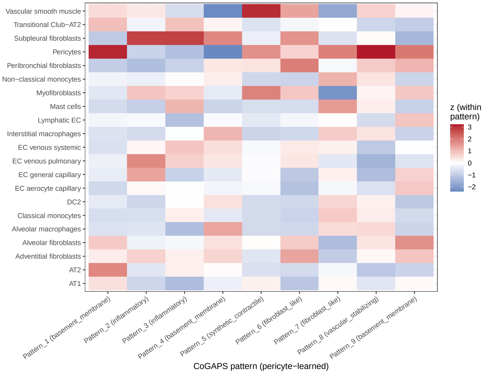
projectR transfer of pericyte patterns onto the niche (nP=9)
