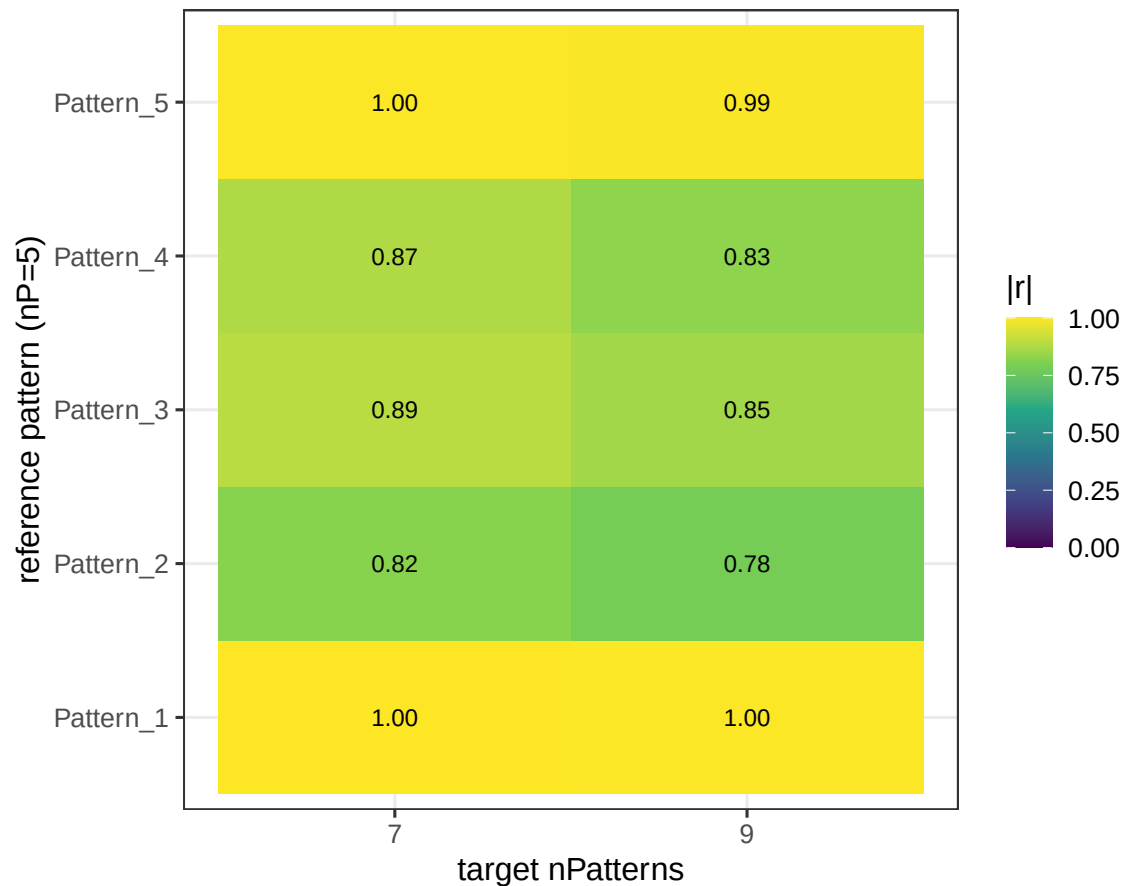
Persistence of nP=5 programs at higher resolution
