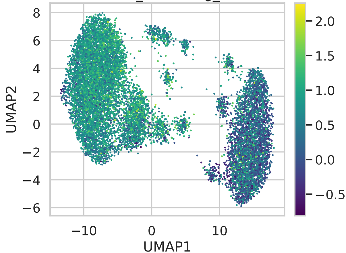
vascular_stabilizing_score
