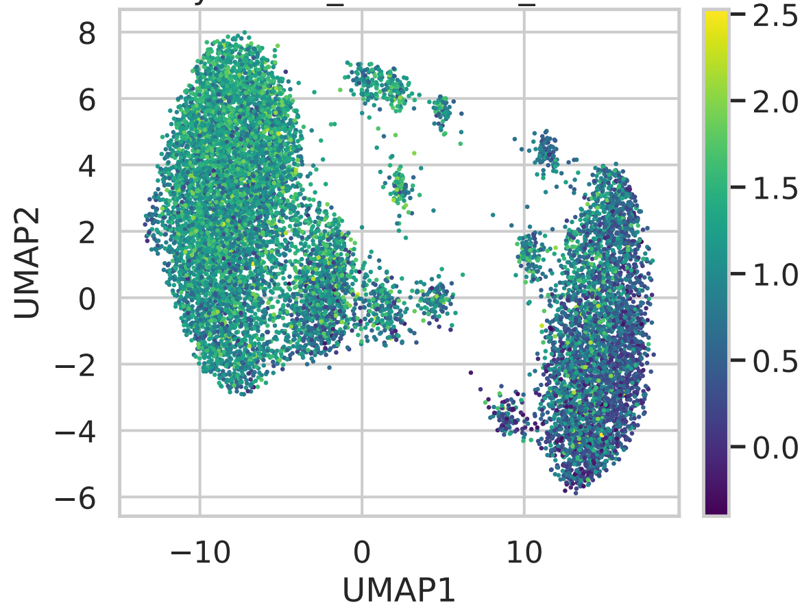
synthetic_contractile_score
