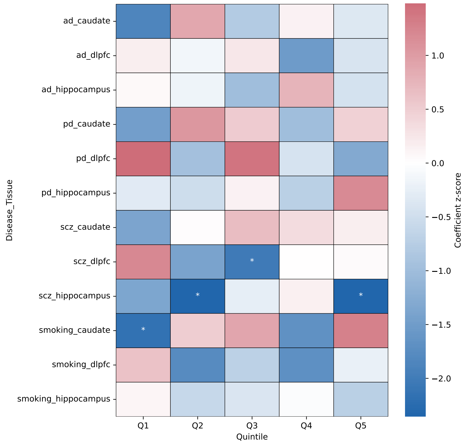
WA-subset Coefficient Z-scores
