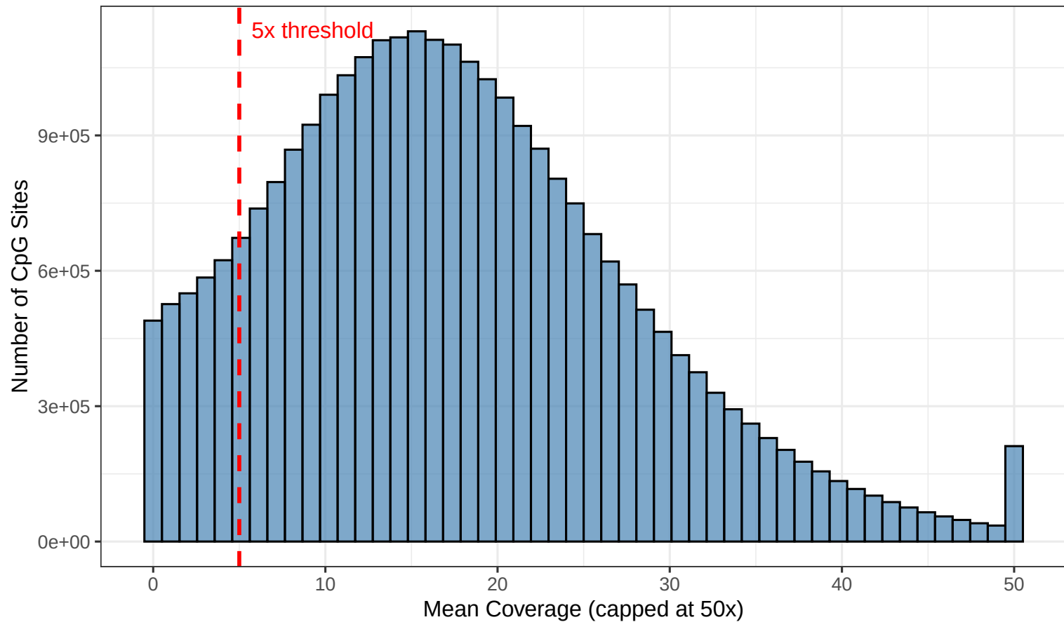
CpG Coverage Distribution: DLPFC
