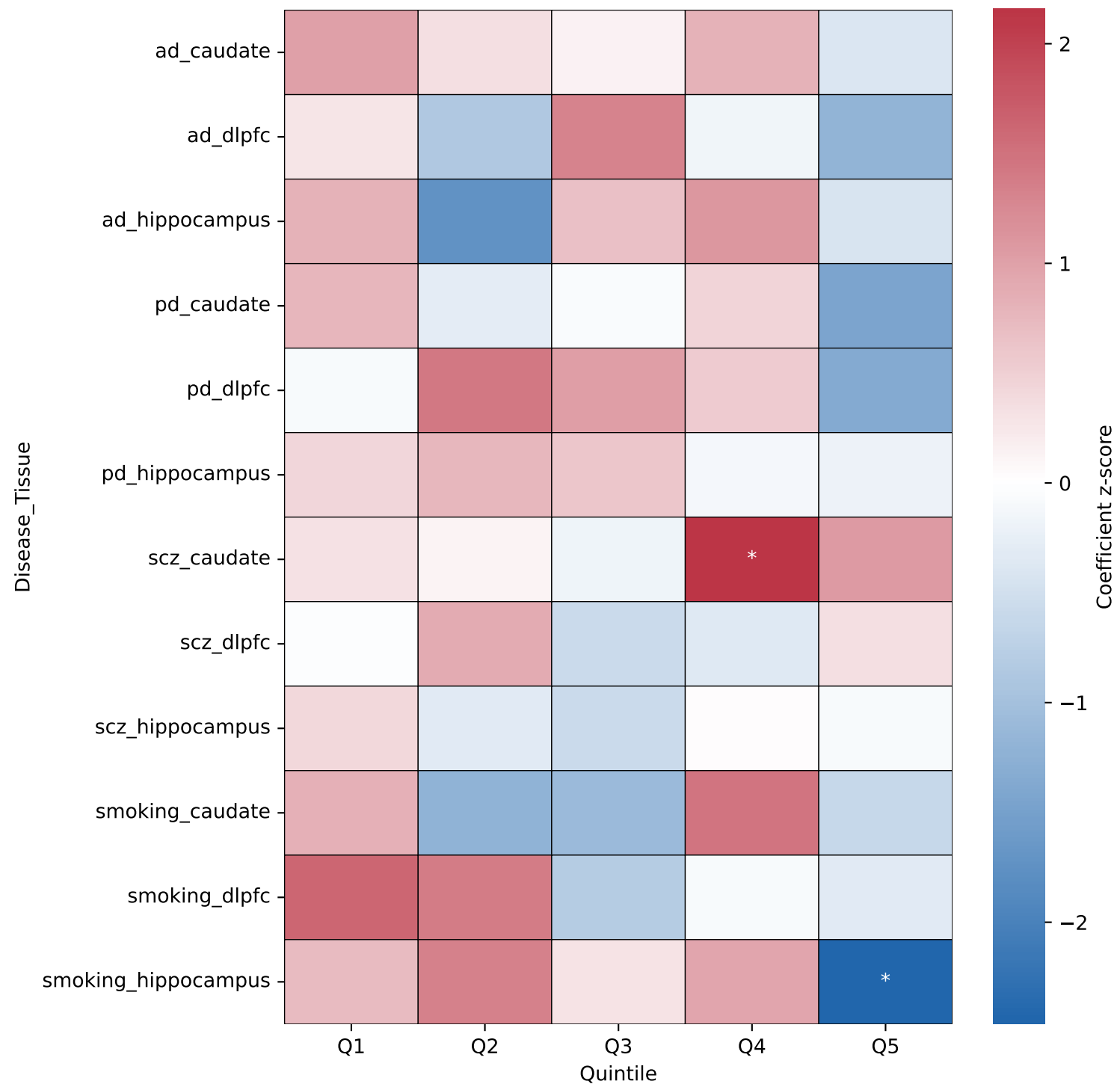
EA-subset Coefficient Z-scores
