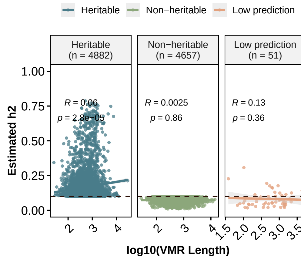
VMR length correlation:DLPFC-AA
