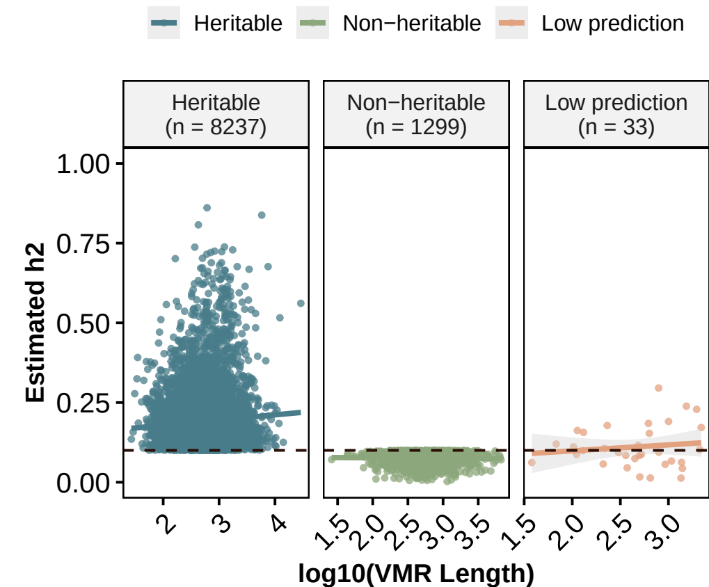
VMR length correlation:DLPFC-EA
