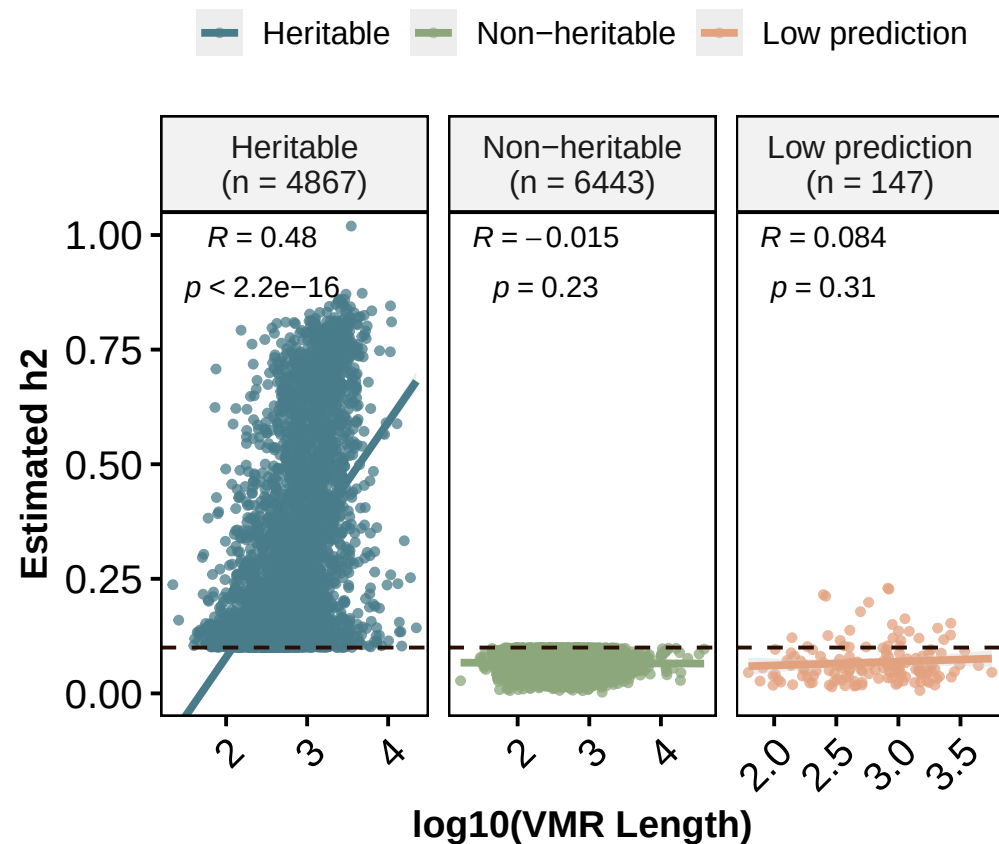
VMR length correlation:Hippocampus-EA
