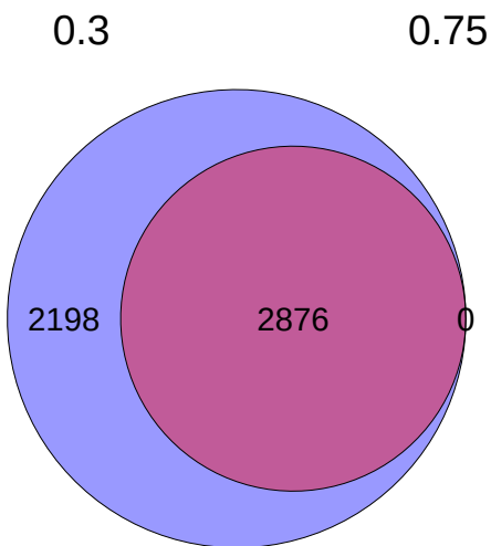
caudate Non-heritable EA
