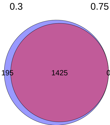
dlpfc Non-heritable EA
