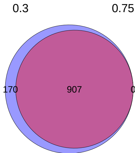
hippocampus Non-heritable EA
