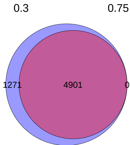
caudate Heritable EA
