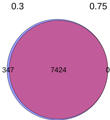
dlpfc Heritable EA
