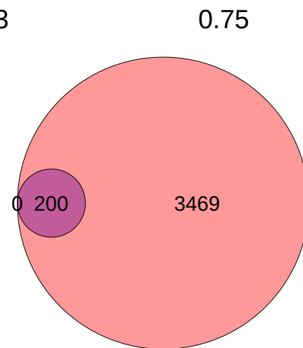
caudate Low prediction EA
