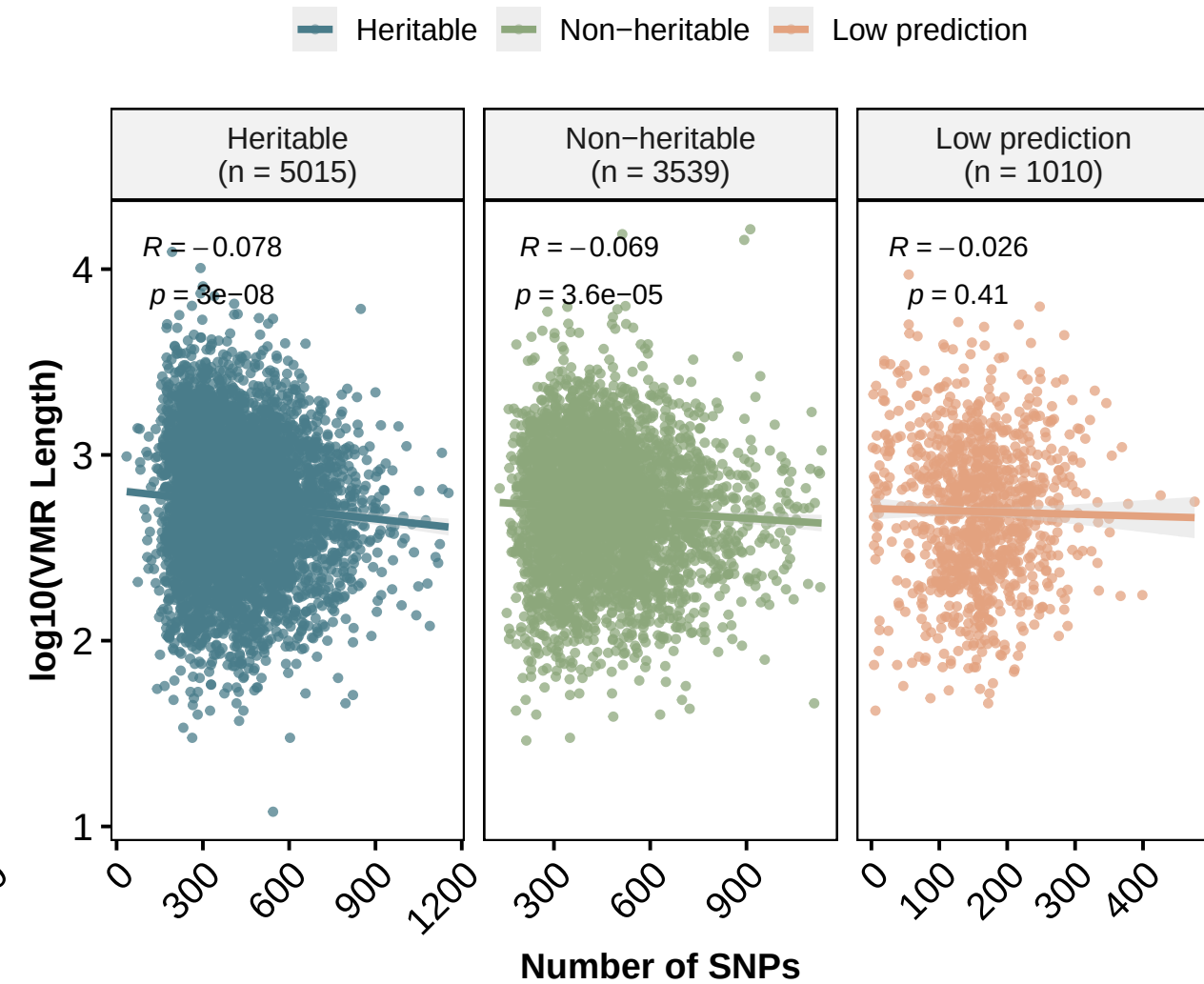
Number of SNPs vs. VMR length: DLPFC
