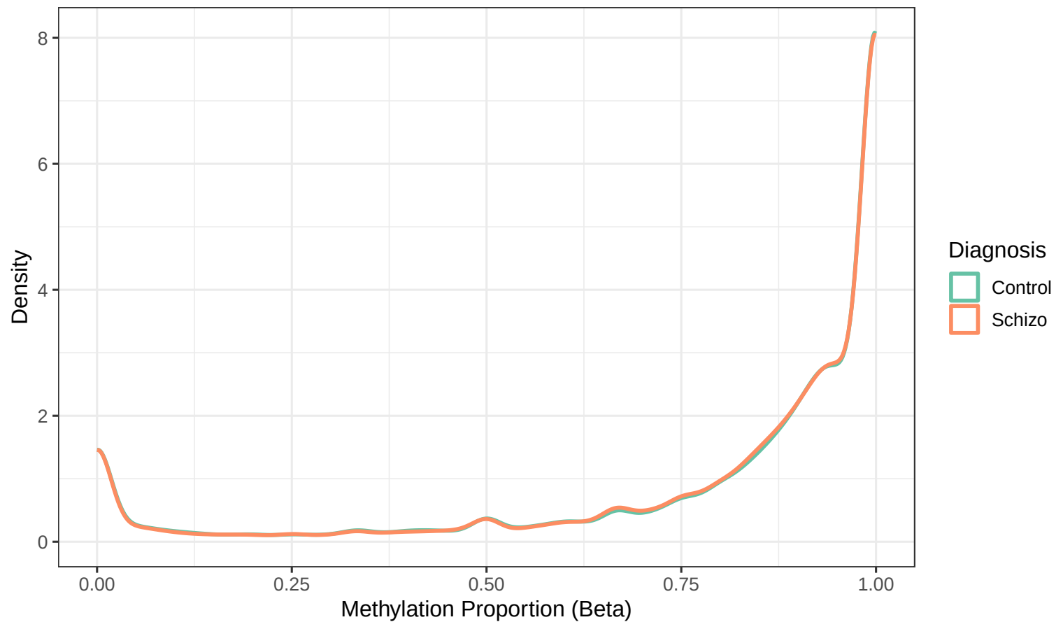
Methylation Distribution by Diagnosis: DLPFC
