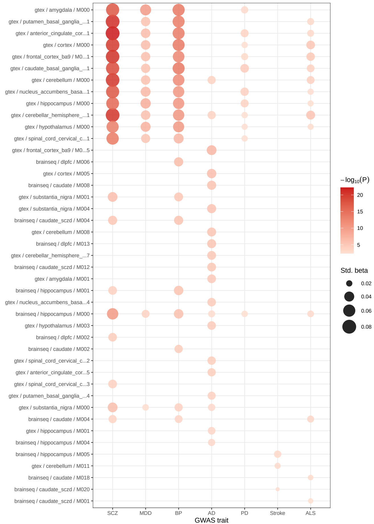
Gene-level WGCNA modules
