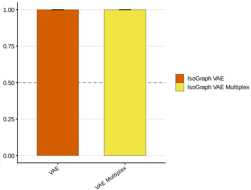
Switch-strength AUROC
