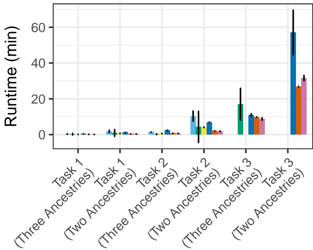
Runtime – CPU
