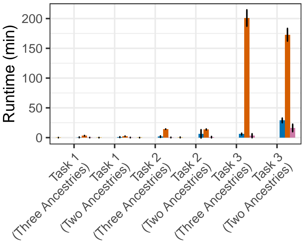
Runtime – GPU
