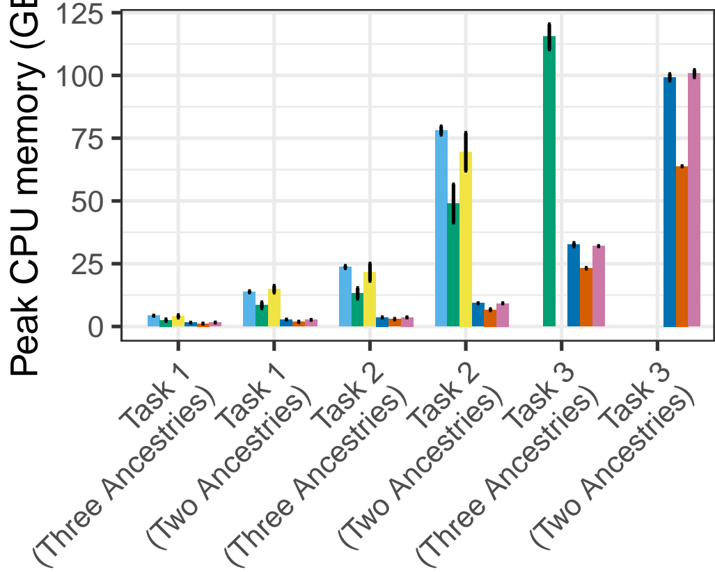
Peak CPU memory – CPU
