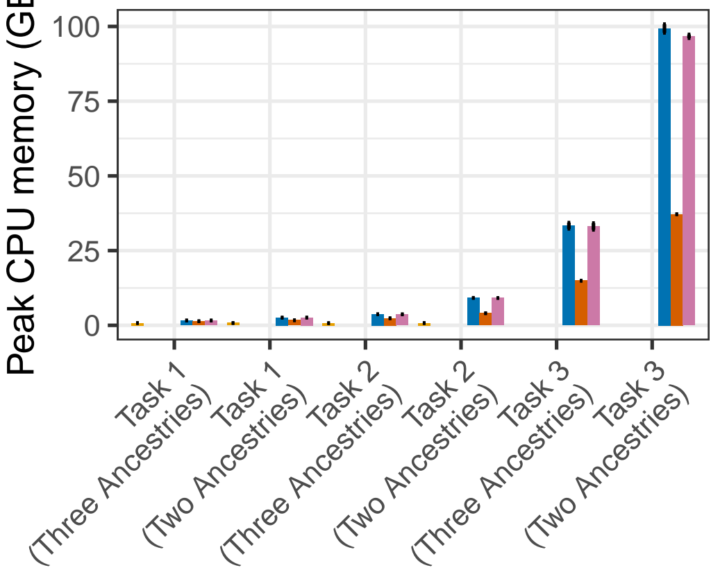
Peak CPU memory – GPU
