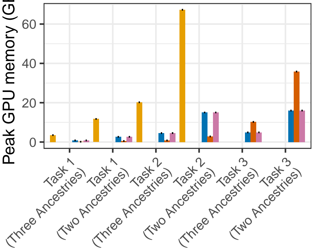
Peak GPU memory – GPU
