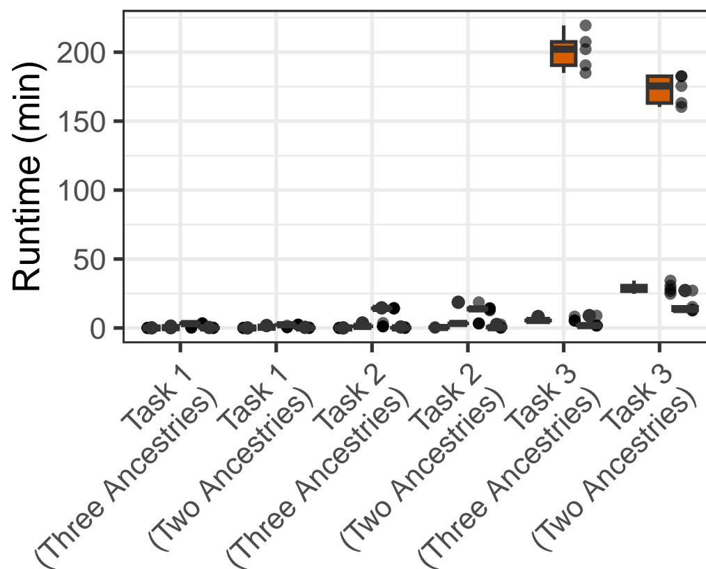
Runtime – GPU
