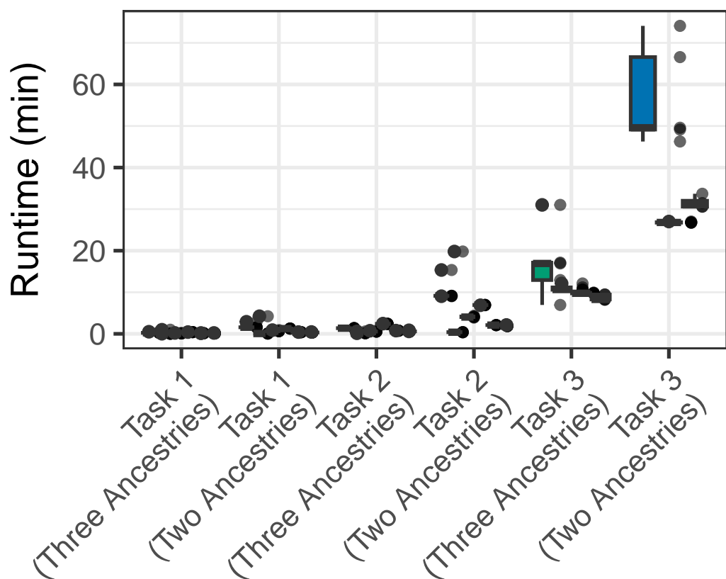
Runtime – CPU
