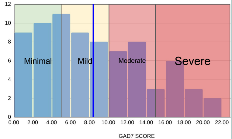
Histogram of GAD7 SCORE
