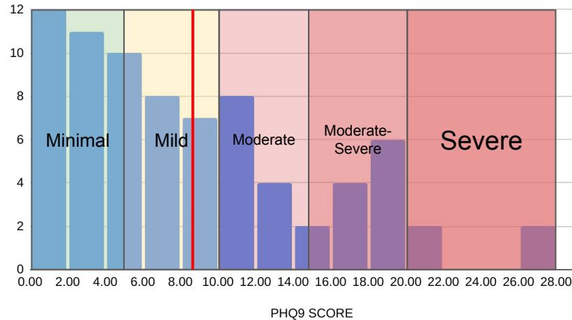
Histogram of PHQ9 SCORE
