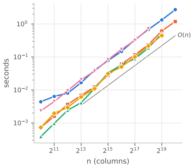
(b) solve with stored factors
