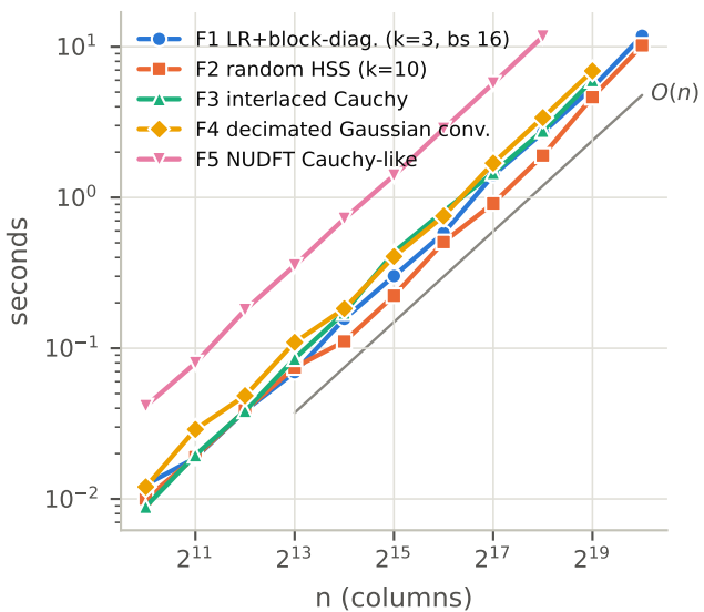
(a) factorization (all levels)
