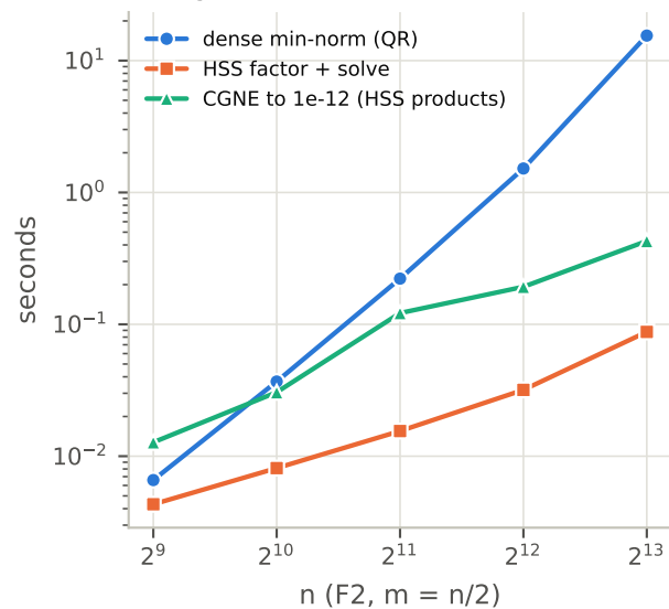
(c) against dense and iterative
