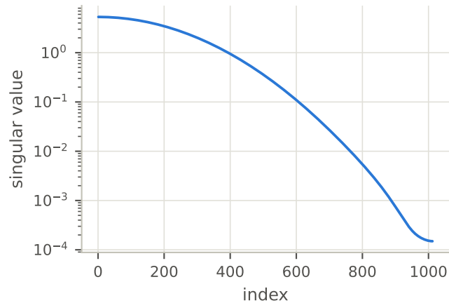
(c) spectrum, \kappa = 3.6\text{e}+04
