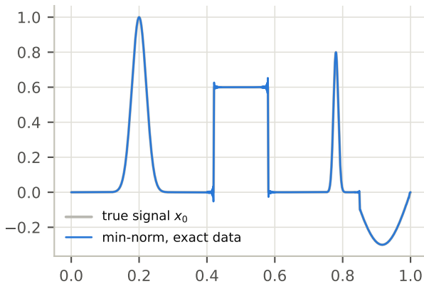
(a) exact data: x^* = P_{\text{Range}(H^*)}x_0
