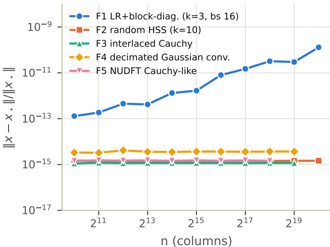
(a) error vs manufactured min-norm solution
