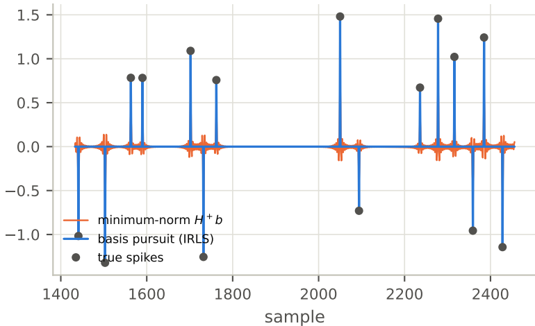
(a) sparse spikes, Ricker wavelet, stride 2
