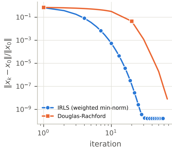
(b) convergence
