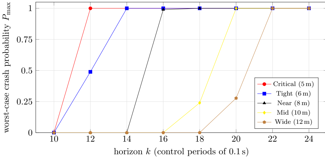
Figure 18: Worst-case crash probability against the horizon for the five car-following scenarios. A larger starting gap delays the rise from 0 to 1.
