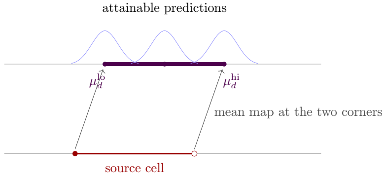
Figure 10: The attainable predictions. The mean map at the two corners of the source cell bounds the predictions; every value between is attained by some state of the cell, and none outside is. Each prediction on the interval carries its own density; three are drawn.
