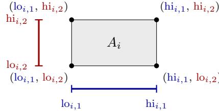
Figure 5: The corners of a cell, for n = 2 . The cell's interval in dimension 1 (blue, below) has the two endpoints \text{lo}_{i,1} and \text{hi}_{i,1} ; its interval in dimension 2 (red, left) has the endpoints \text{lo}_{i,2} and \text{hi}_{i,2} . Each corner pairs one blue endpoint with one red endpoint, as its label shows; two choices per dimension give 2^n = 4 corners.
