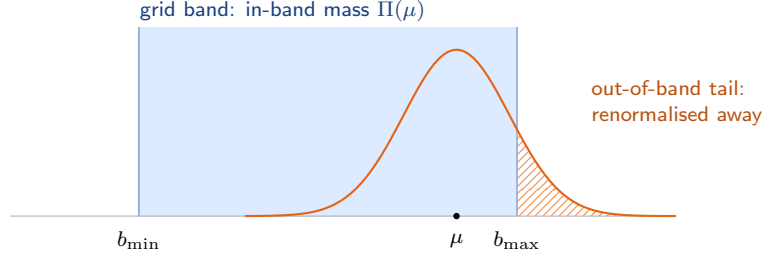
Figure 13: Truncation of the stochastic tail. The grid band [b_{\min}, b_{\max}] covers a bounded interval of a stochastic dimension, while the Gaussian factor has unbounded support. The fraction of mass inside the band, \Pi(\mu) , depends on the prediction \mu ; the out-of-band tail is renormalised away, conditioning the kernel on the band.
