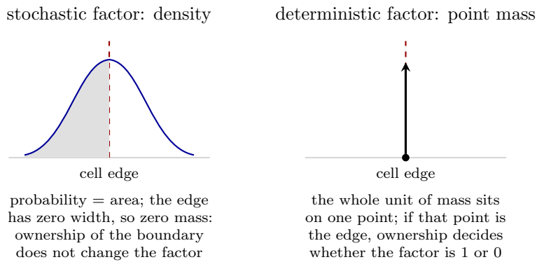
Figure 14: The two factor types of the product kernel. A density factor (left) assigns zero probability to any single point, so which cell owns a shared boundary does not affect its value. A point-mass factor (right) concentrates the whole unit of mass on one point; when the image lands exactly on a shared boundary, the half-open convention of Section 4.1 determines which cell receives the mass, which is why the upper inequality in (17) must be strict.
