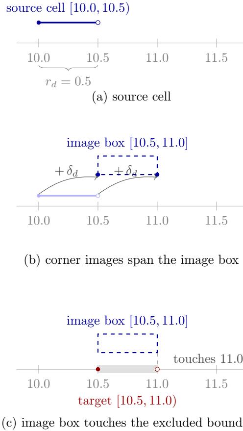
Figure 8: A touching image from an aligned step. The step \delta_d = r_d = 0.5 sends both corners of the source cell onto grid lines, so the image box touches the excluded upper boundary of the target and the factor is [0, 1] .
